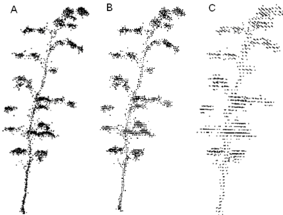
Fig. 1: Tree point clouds of an exemplary juvenile beech tree. With increasing grid space the resolution of the tree model decreases and finer contours disappear. Tree height was about 41 cm. A) Point cloud as created from the original scanner data (3411 points). B) 0.5-cm point cloud grid computed with Mathematica (2296 points). C) 1-cm point cloud grid (1105 points).
