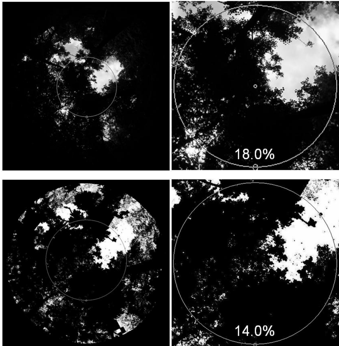
Fig. 5: Comparison of a hemispherical photograph taken from the ground (top) and its voxel-based simulation derived from six scans (below). On the left side is the whole scene, on the right the more restricted sections of the two images enlarged to allow for better comparison. Circles indicate the 30^\circ zenith angle in which the analysis was done. Percent values indicate canopy openness within the analyzed circle.
