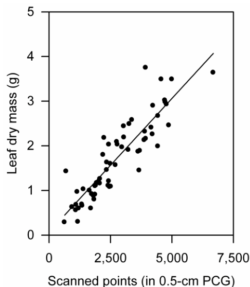
Fig. 2: Relationship between leaf dry mass per tree measured by harvesting and the number of points in a 0.5-cm point cloud grid created by laser scanning ( p < 0.001 ; R^2 = 0.81 ; n = 60 ).
