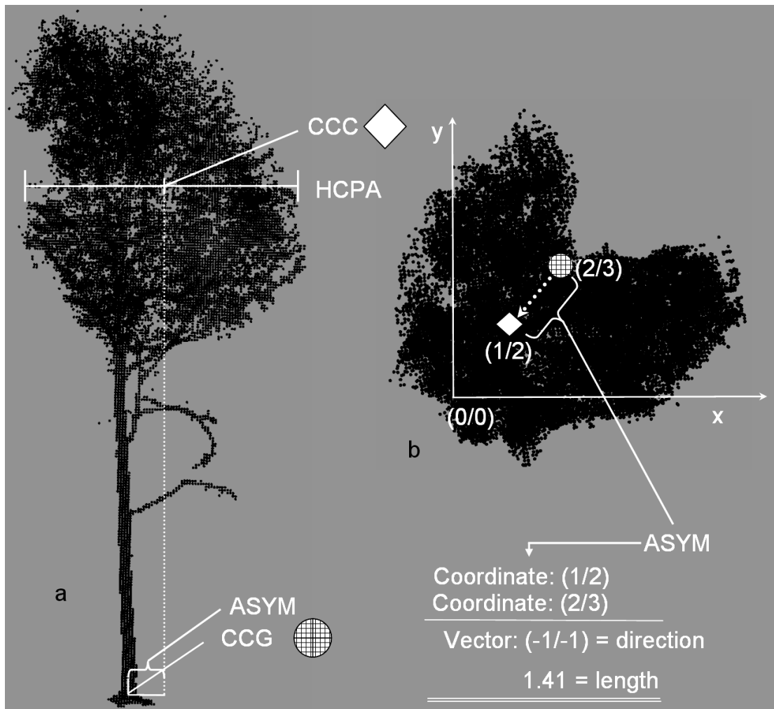
Fig. 5: Graphical presentation of structural parameters used to quantify the degree and direction of the asymmetry of a canopy. a) Side view on a tree with the asymmetry (ASYM) being equalled with the horizontal distance between CCG and CCC. b) Top view on the same tree with CCC and CCG marked including their coordinates. The difference between the x- and y-values can be expressed as a vector, with the length of the vector being the measure for the degree of asymmetry.
