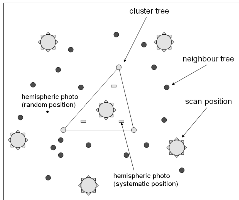
Fig. 1: Example tree cluster with the three cluster trees and additional surrounding trees and position of laser scans and hemispheric photos.
