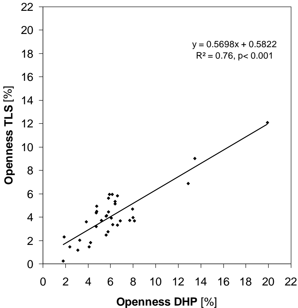
Fig. 4: Relationship between the calculated canopy openness obtained from terrestrial laser scanning ('TLS', calculated with Mathematica) and openness calculated from digital hemispherical photography ('DHP', calculated with Gap Light Analyzer) for a set of 35 scan sessions taken in both study areas.
