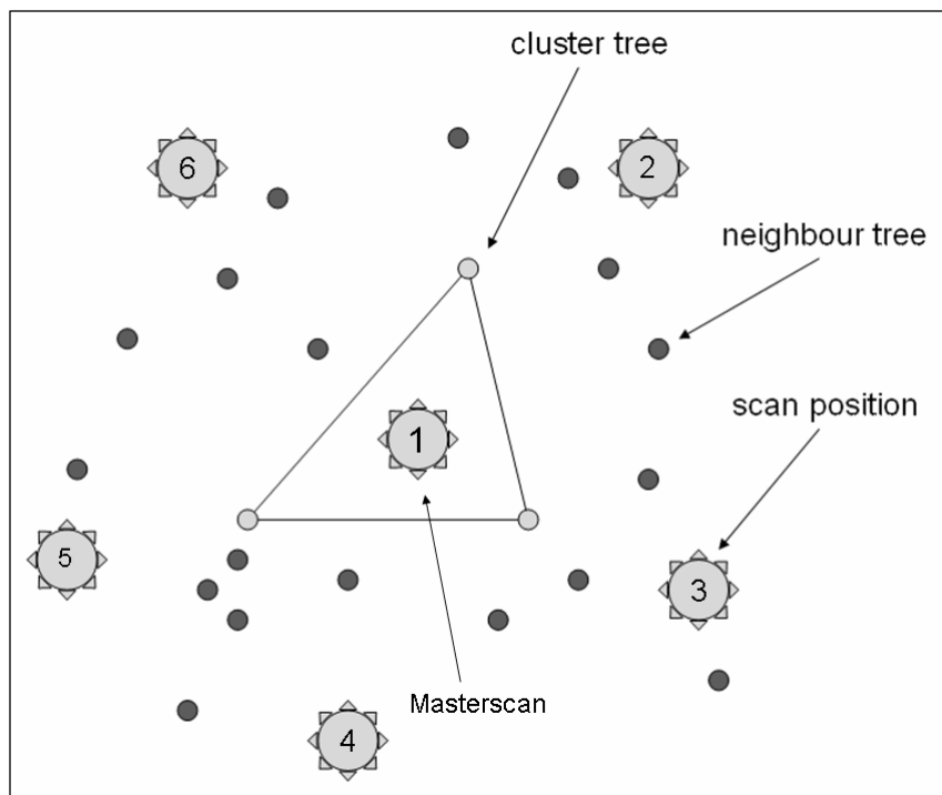
Fig. 3: Scan design as performed on all hundred tree diversity clusters.
