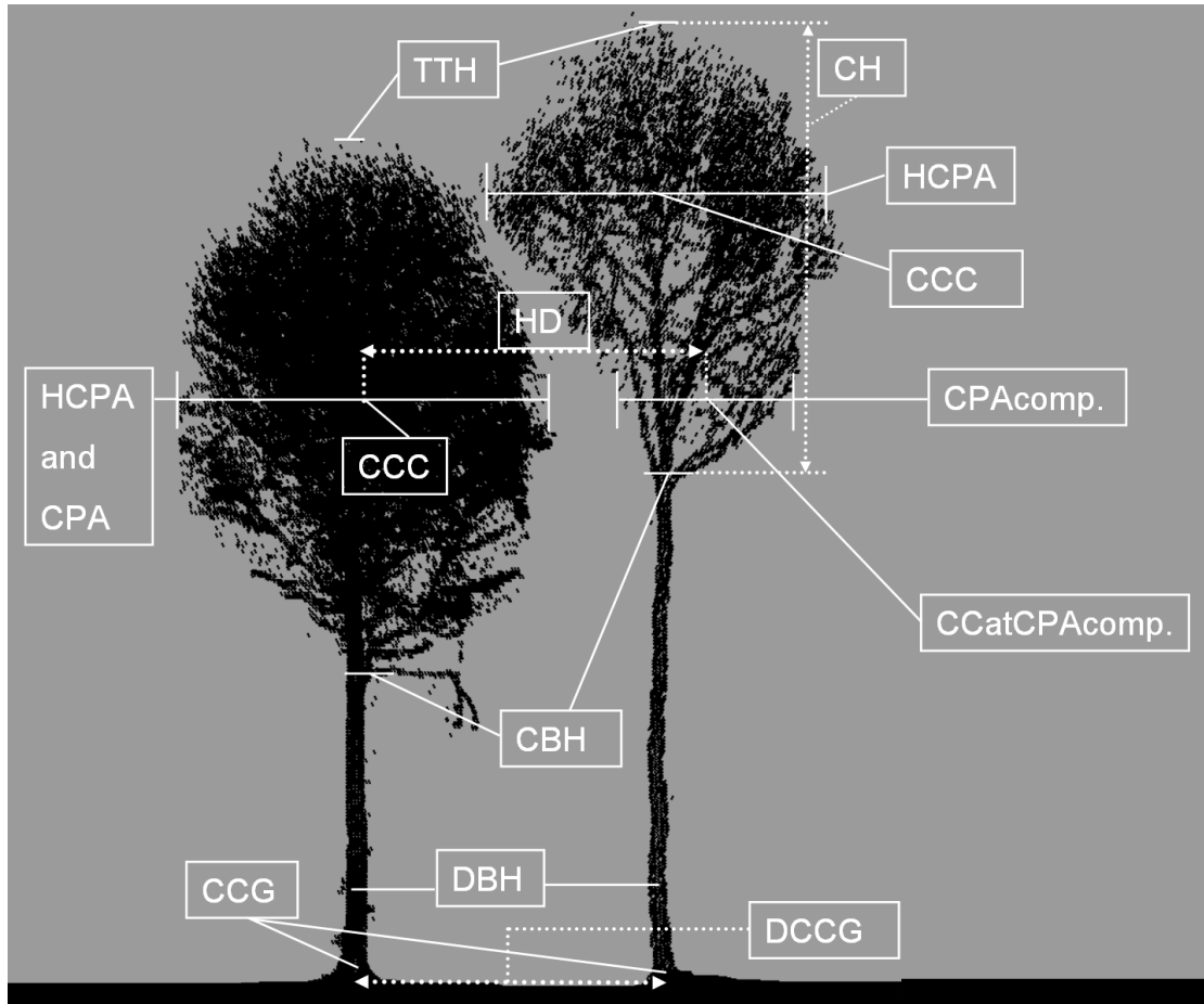
Fig. 3a: Graphical presentation of the most important structural parameters derived for an exemplary focal tree and an exemplary neighbor tree: total tree height (TTH), diameter at breast height (DBH), crown base height (CBH), crown height (CH), coordinates of the centre of the stem at ground level (CCG), height of maximum crown projection area (HCPA), maximum crown projection area (CPA), centre of the crown at the height of maximum crown projection area (CCC), crown projection area at the height of the maximum crown projection area of the focal tree (CPAcomp, only for neighbor trees), centre of the crown at the CPAcomp (CCatCPAcomp), horizontal distance between the CCC of the focal tree and the CCatCPAcomp. of the competitor (HD) and horizontal distance between the CCG of the focal tree and the CCG of the neighbor tree (DCCG).
