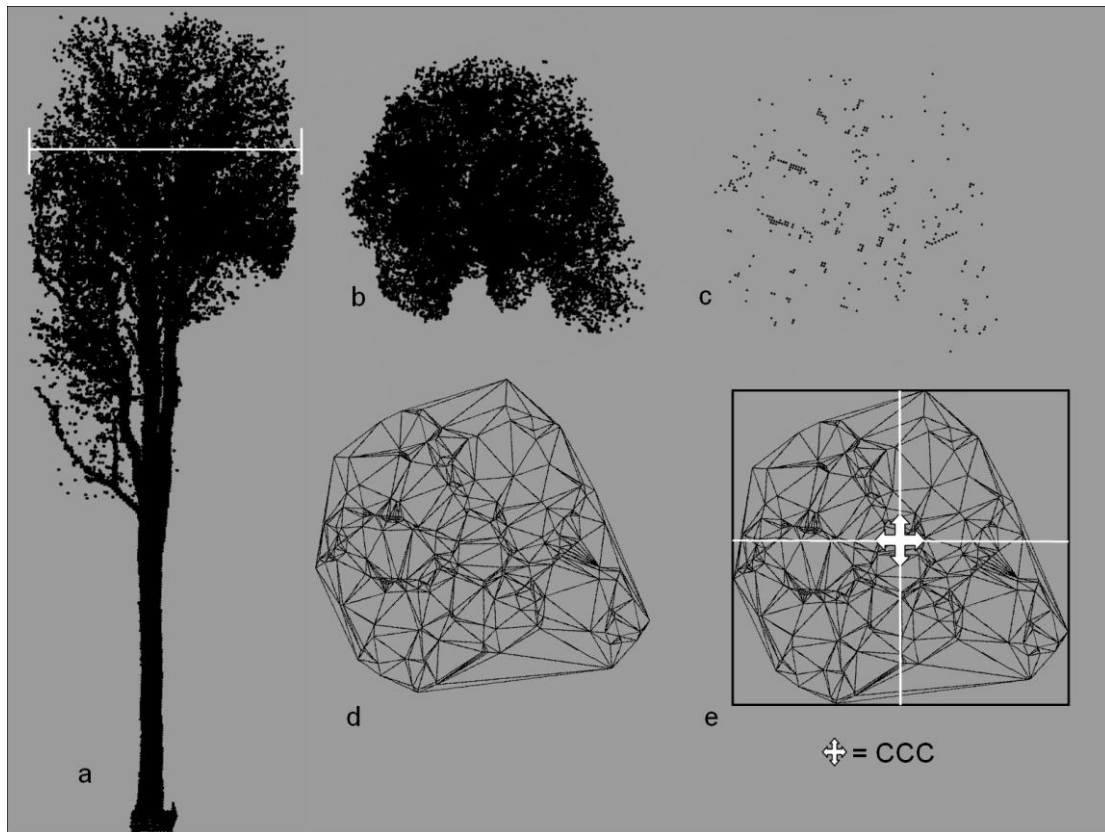
Fig. 3b: Graphical presentation of the maximum crown projection and the centre of the crown at the height of the maximum crown projection area. All images are based on the 10-cm voxel-model with only the centre-points of the voxels shown. a) 3-D point cloud of a tree with the height of the maximum crown projection area highlighted with a white line, side view. b) The same tree as in a) but in top view, showing the shape of the crown as visible from above. c) All voxel centre-points in the layer of the height of the maximum crown projection area. d) Outer hull of the point cloud in c. as used to calculate the maximum crown projection area. d) Centre of the crown at the height of the maximum crown projection area which is derived from placing a rectangle on the outermost edge points of the canopy volume and marking the centre of the rectangle.
