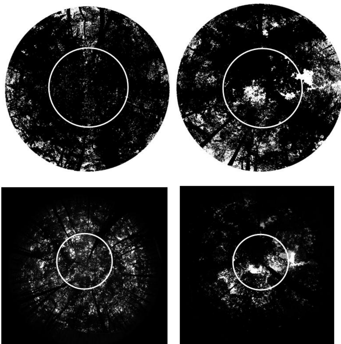
Fig. 6: Typical hemispheric view of the Thiemsburg (left) and the Lindig (right) canopies. Simulation (top) and photograph (bottom) are compared up to 30^\circ zenith angle (indicated by the white circles).
