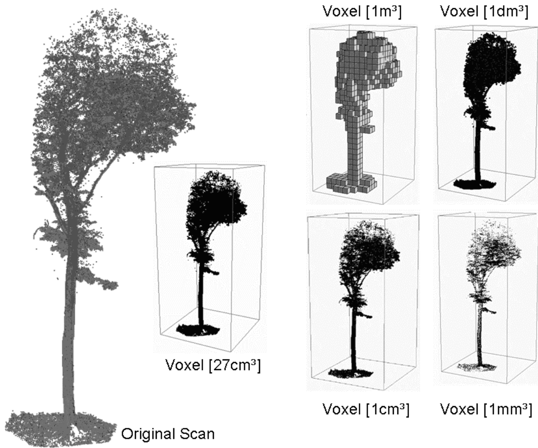
Fig. 3: (left) Point cloud of a single tree ( Fagus sylvatica ) as produced by six laser-scans. (right): Models of the same tree based on voxel sizes from one m 3 to one mm 3 . (centre): voxels of 27 cm 3 as used in the simulation.
