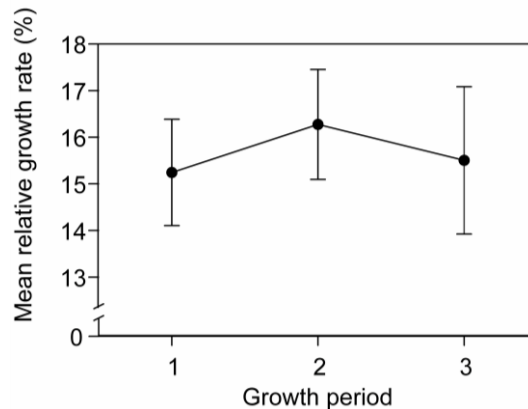
Fig. 5: Mean relative growth rate (%) of 36 experimental trees that were measured on four occasions during 77 days. Error bars show the standard error ( n = 36 ). Growth was measured as the relative biomass increase during three periods: Period 1 : July 13, 2009 - July 27, 2009; Period 2 : July 27, 2009 - September 9, 2009; Period 3 : September 9, 2009 - September 28, 2009.
