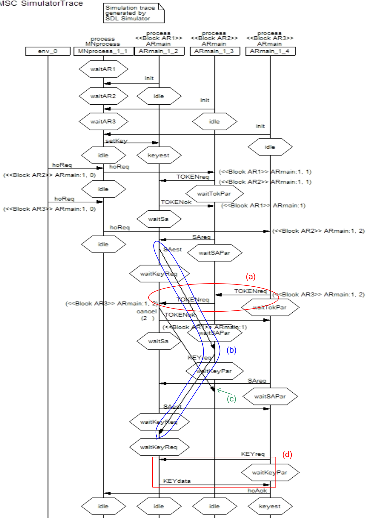
Figure 32: MSC - Handover from AR1 to AR2, AR3
