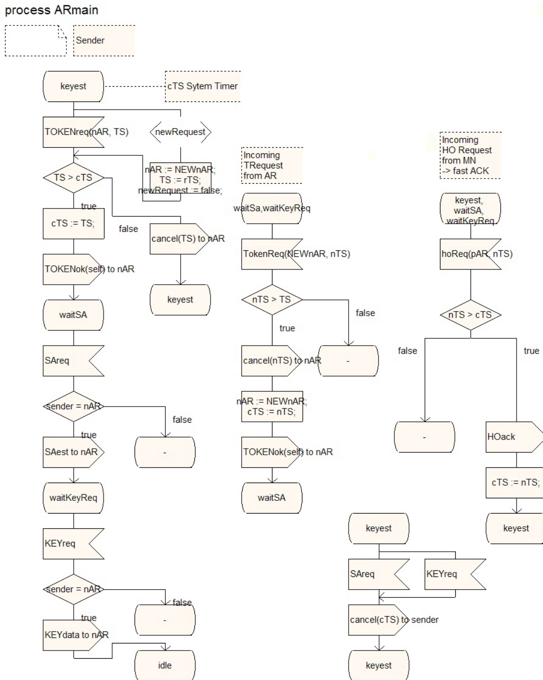
Figure 29: SDL Process Model of the IDKE-AR Sender Part
