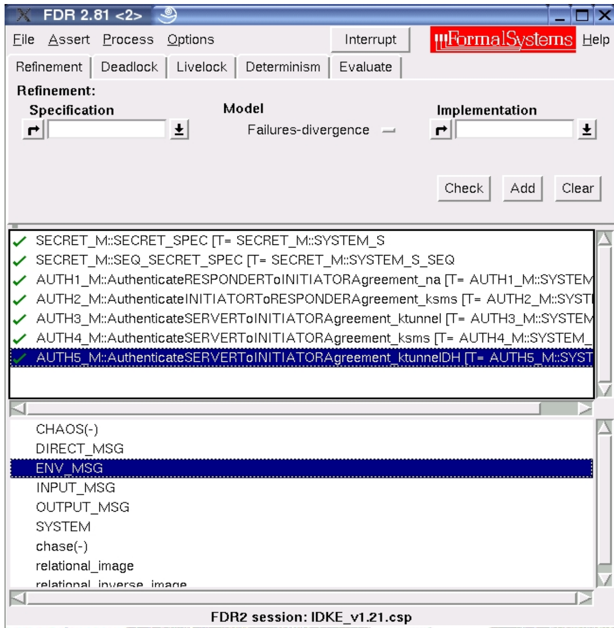
Figure 52: FDR Screenshot – Output for the Final Version
