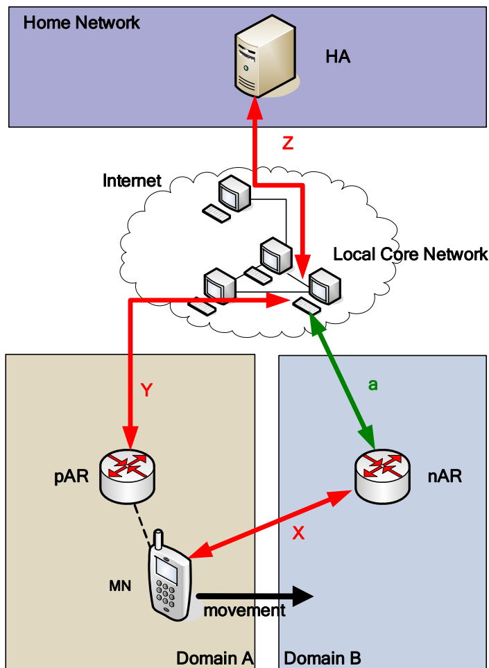
Figure 44: Network Topology
