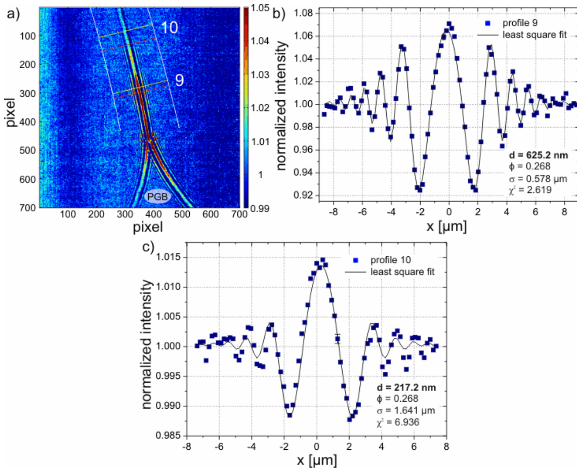
Figure 3.7: (a) Diffraction pattern of the transition region during the "zipper-like" effect of a microfluidic lipid membrane close to the Plateau-Gibbs border (PGB) (Monoolein-squalane / water, z_{eff} = 94.21 nm). The Fresnel fringes disappear in regions where the membrane has already thinned and only a single maximum is left. (b) Profile 9 , along with a reasonable least-squares fit, showing a large thickness at the position of a thick, domain of residual solvent. (c) Profile 10 , which is located close to the bimolecular membrane region, cannot be fitted comparably accurately due to a notable contribution of the PGB to the diffraction pattern.
