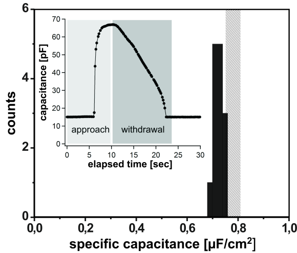
Figure 1.6: Measurements of the specific capacitance of a bilayer membrane of mono-olein in squalane. The black histogram represents the measured values. The grey bar indicates the literature values for oil-free mono-olein membranes. Inset: trace of capacitance measurement upon approach and withdrawal of two droplet surface to/from each other.
