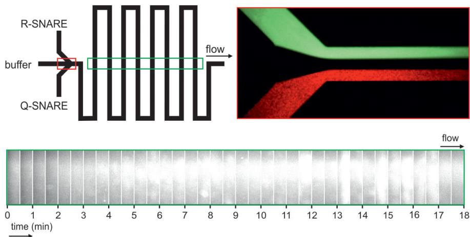
Figure 2.5: Channel geometry of a microfluidic device for membrane fusion. Top left: It consists of a cross geometry when the two SNARE populations are mixed. Top right: Mixing of SNARE liposome populations is achieved by hydrodynamic flow focussing. Bottom: Images of the acceptor fluorescence in the different turn segments of the channel are recorded as shown. The fusion is monitored by recording the average intensity of each time window. It can be clearly seen that as time proceeds (i.e. in the direction of the flow), the brightness of the images increases. This is due to the increase in the FRET signal that follows the fusion event.
