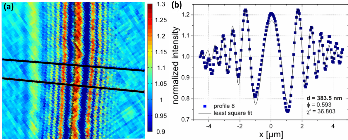
Figure 3.5: a) Diffraction pattern of a microfluidic bilayer membrane prepared from a Monoolein-squalene solution / water at an effective propagation distance of 29.67 mm. The Fresnel fringes are highly visible at high deflection angles. Glue residues at the surface of the self-adhesive kapton window material produce parasitic features in the image. b) The profile between the black lines is extracted from the region of interest (ROI) in (a). Due to planar sample geometry it can be fitted using a symmetric phase slit model 96 , which is characterized by the phase shift \phi and the thickness d .
