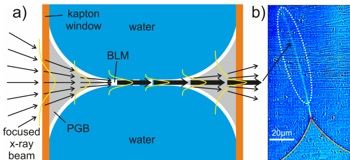
Figure 3.8: (a) Schematic representation of the “focusing” effect of the Plateau-Gibbs border. This results in an intensity maximum in (b) at the position of the thinned membrane. Images of (b): data: hunt01-7150 , background: hunt01-10049 .
