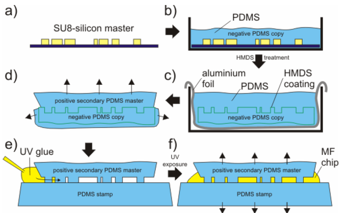
Figure 3.2: To protect the SU8 masters (a) a three step copying technique is used for the microfluidic chip production. After preparing a negative PDMS copy of the channel structure (b) its surface is treated with HMDs and a secondary (positive) PDMS master is taken (c). This secondary master is separated from the surrounding PDMS (d) and placed on a flat PDMS stamp (e). The spaces in between are filled with UV curable glue and after 5 to 10 minutes of UV light exposure the microfluidic chip can be peeled off (f).
