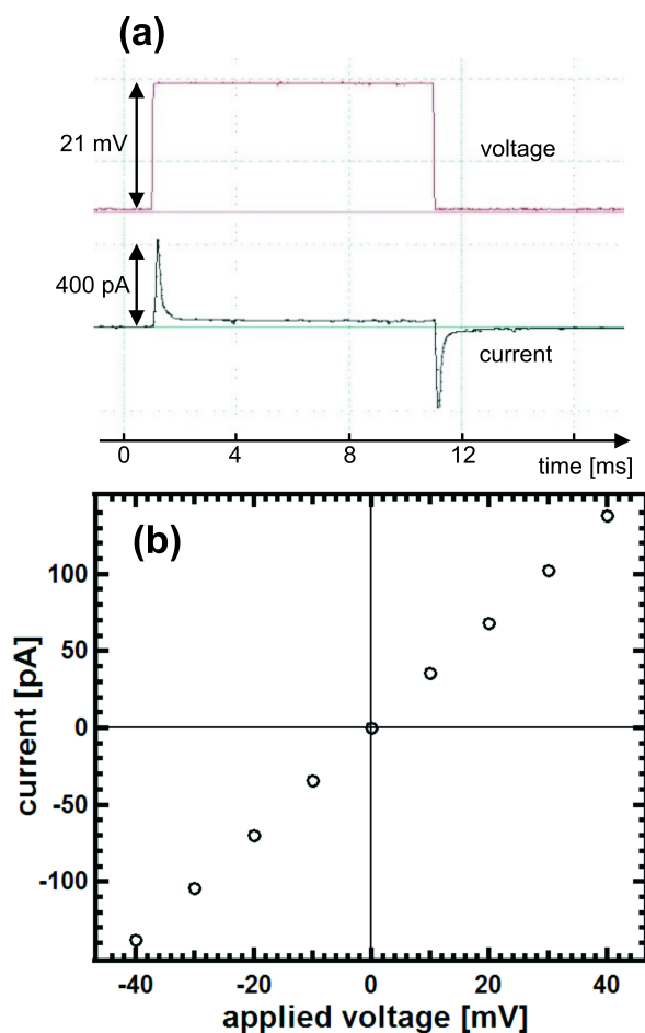
Figure 1.10: Electrical properties of mono-olein membranes formed and suspended in a micro-fluidic channel. (a) A square wave voltage is applied (top). The current trace (bottom) shows distinct peaks indicating the charging current of the membrane capacitance. (b) The small offset observed in the current trace in (a) is plotted as a function of applied voltage. We clearly see an ohmic behavior, which probably stems from ionic impurities.
