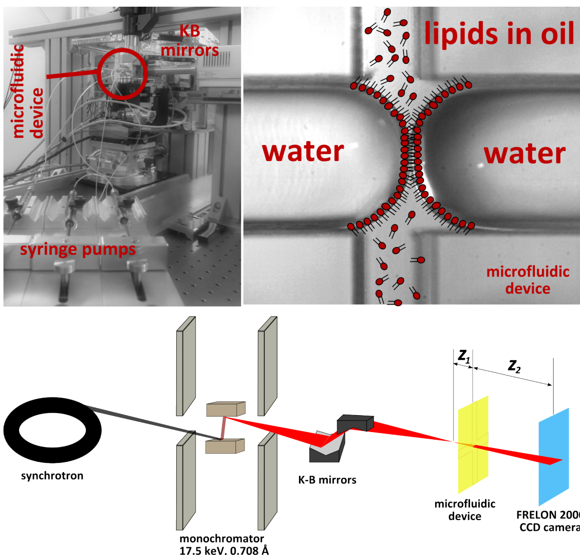
Figure 3.1: A schematic of the synchrotron setup, at the ID22 (ESRF) beamline, for imaging a microfluidic lipid bilayer. A microfluidic device in which a lipid bilayer can be formed by two water droplets suitably covered by a monolayer of lipid.
