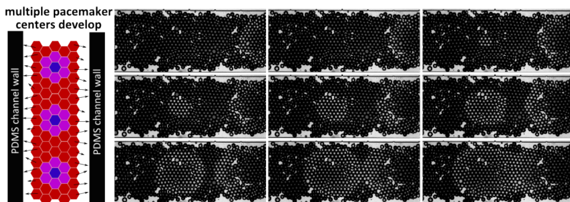
Figure 4.10: Formation of target waves with multiple pacemaker centers in a oscillator network confined in a PDMS microchannel. Left: Schematic of the oscillators in a PDMS channel. PDMS, in addition to the oil phase, absorbs the excitatory and inhibitory components of the BZ at the edges (shown by the arrows). Right: Two target wave patterns seen in the channel. One target wave is forming at a pacemaker center clearly visible. The center of target pattern coming in from the right is not visible.
