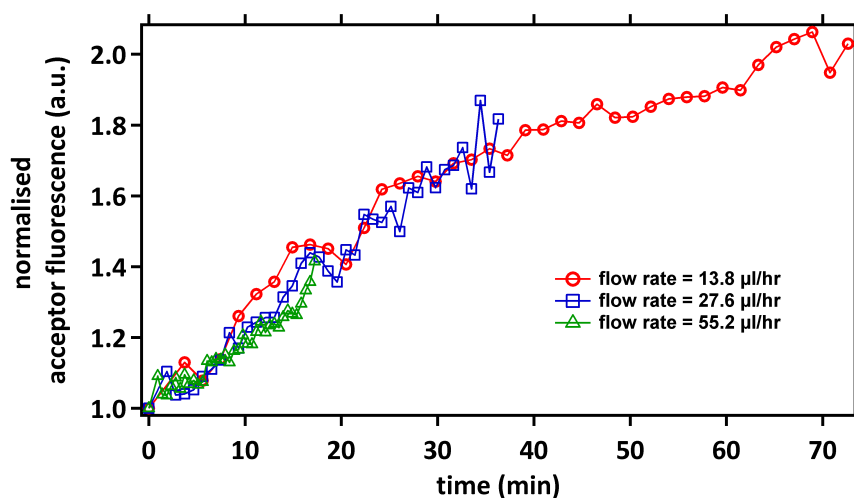
Figure 2.6: Flow rate control of time axis in the microfluidics experiments. As we increase the flow rate, thus shortening the time along the channel, we see that the fusion of the membranes proceeds only until that time point (green curve). We then see that these time points depend linearly on the flow rate within the channel.
