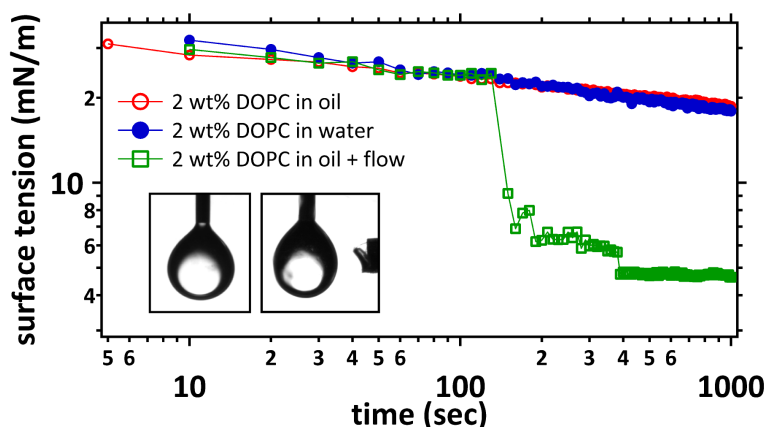
Figure 1.4: Effect of flow on the evolution of interfacial tension. Data: courtesy of Jean-Baptiste Fleury
