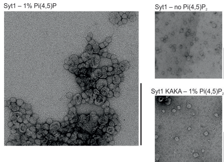
Figure 2.12: In the absence of Ca^{2+} , synaptotagmin-1 leads to liposome clustering. This clustering is mediated by the electrostatic binding of synaptotagmin-1 to anionic lipids in the liposomes.
