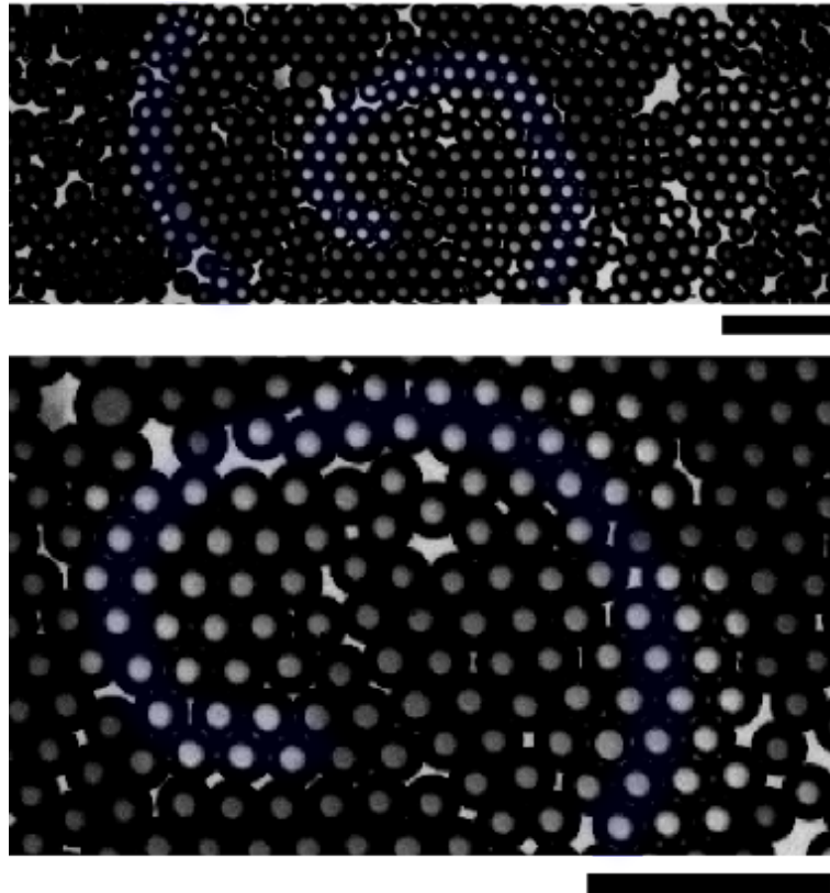
Figure 4.12: Formation of spirals in oscillator networks. Top: A spiral can be seen clearly in the oscillator population. Bottom: Image of the network at higher magnification revealing the lack of perfect local connectivity for each droplet. Scale bar is 150 microns.
