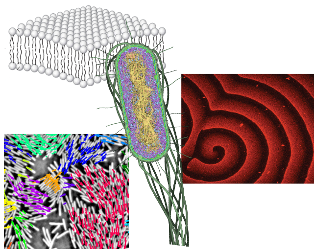
Figure I.1: Center: A cartoon of a cross section through a single bacterial cell. Clockwise from top: The cell membrane is primarily a lipid bilayer, acting as a scaffold for various proteins. Cytoplasmic bacterial proteins interact with the lipid membranes to self organize, giving rise to functions such as cell division and also a rich variety of patterns 1 . Flagellar motors in the cell wall drive bacterial motion and in a group, locomoting cells spontaneously orient in swarming clusters 8 . (Figures are adapted with permission from 1,8,9 )
