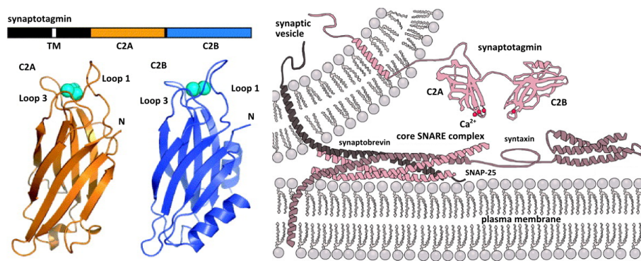
Figure 2.2: Synaptotagmin-1 is the Ca^{2+} sensor for membrane fusion. Left: Synaptotagmin has a single transmembrane domain (TM) which embeds into the lipid bilayer of the synaptic vesicle. This is followed by a large cytoplasmic domain, which ‘sticks out’ into the cytoplasm of the cell. This domain is comprised of two parts the C2A and C2B which have 2 and 3 sites, respectively, for binding Ca^{2+} ions. Right: By the current understanding of the fusion process, the SNARE proteins are nucleated i.e. they are primed for fusion via coiling but fusion is somehow arrested. In this picture of fusion, the synaptotagmin acts downstream of the SNARE coiling. (Reproduced with permission from 61 )
