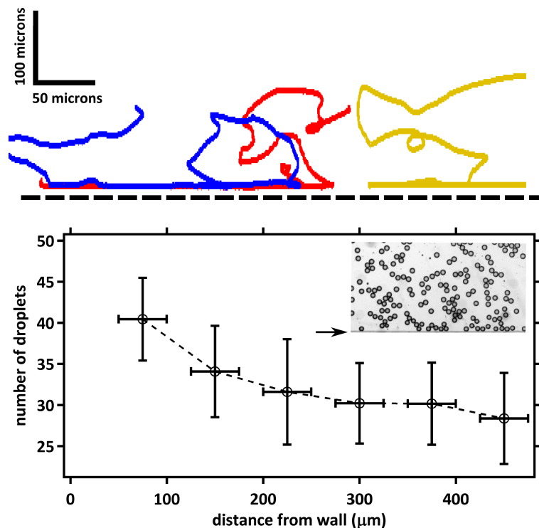
Figure 6.7: Droplet squirmers have attractive interactions with walls. Top: Representative squirmer paths (for 3 different squirmers) near a wall (black dashed line). Bottom: The number of droplets as a function of the distance from the wall for an experiment as shown in the inset. The average droplet diameter is 50 microns and the black arrow points to the wall in the image. Each point on the curve is an average over 1500 time points.
