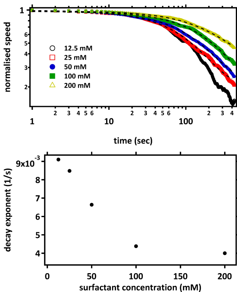
Figure 5.8: The decay of the swimmer speed with time. Top: The normalised speed of the squirmers for various surfactant concentration as a function of time. The normalisation is done with the initial (peak) speed at each concentration. The decay of the velocity is different for each surfactant concentration. The black dashed lines are exponential fits to the data. Bottom: The decay exponent of the normalised speed as a function of surfactant concentration.
