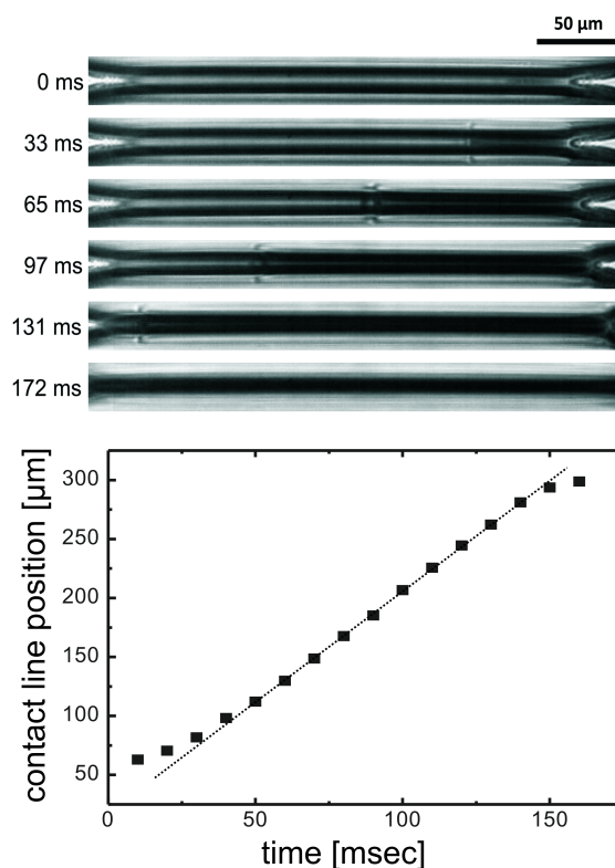
Figure 1.7: Time-resolved micrograph of membrane formation in a micro-fluidic system. Top: time-lapse images of three-phase contact line moving across the oil lamellae while membrane is forming. The total diameter of the membrane is 300\ \mu\text{m} . Bottom: Three-phase contact line position as a function of time. The slope of the dotted line is 1.9\ \text{mm/s} .
