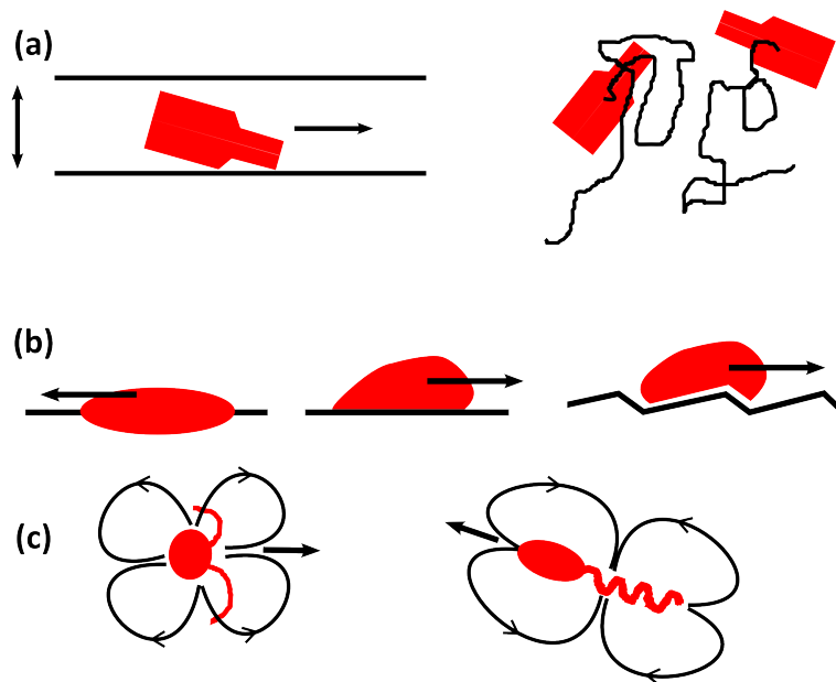
Figure 5.1: The three classes of SPPs (a) Shaken granular media, is comprised of an asymmetric unit vibrated on (or between two) plates resulting in a quasi two dimensional motion (black lines in right image represent object paths) (b) Striders, which move on a surface via modification of the contact properties of the SPP and surface (c) Swimmers, which move in a surrounding fluid, create well defined hydrodynamic flow fields (black lines) around them. In all figures, black arrows indicate direction of motion.
