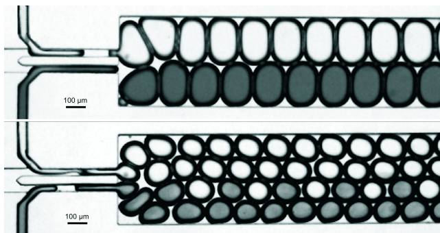
Figure 1.3: Gel emulsions of water in oil generated by step emulsification, forming rafts in a wider channel. The channel width is 500\ \mu\text{m} , the volume fraction of the aqueous phase is 0.75. The elementary cells of such rafts can be quite complex, as the lower example shows. Controlled rearrangement of these configurations are possible by appropriately chosen channel geometries 33,39,41 .
