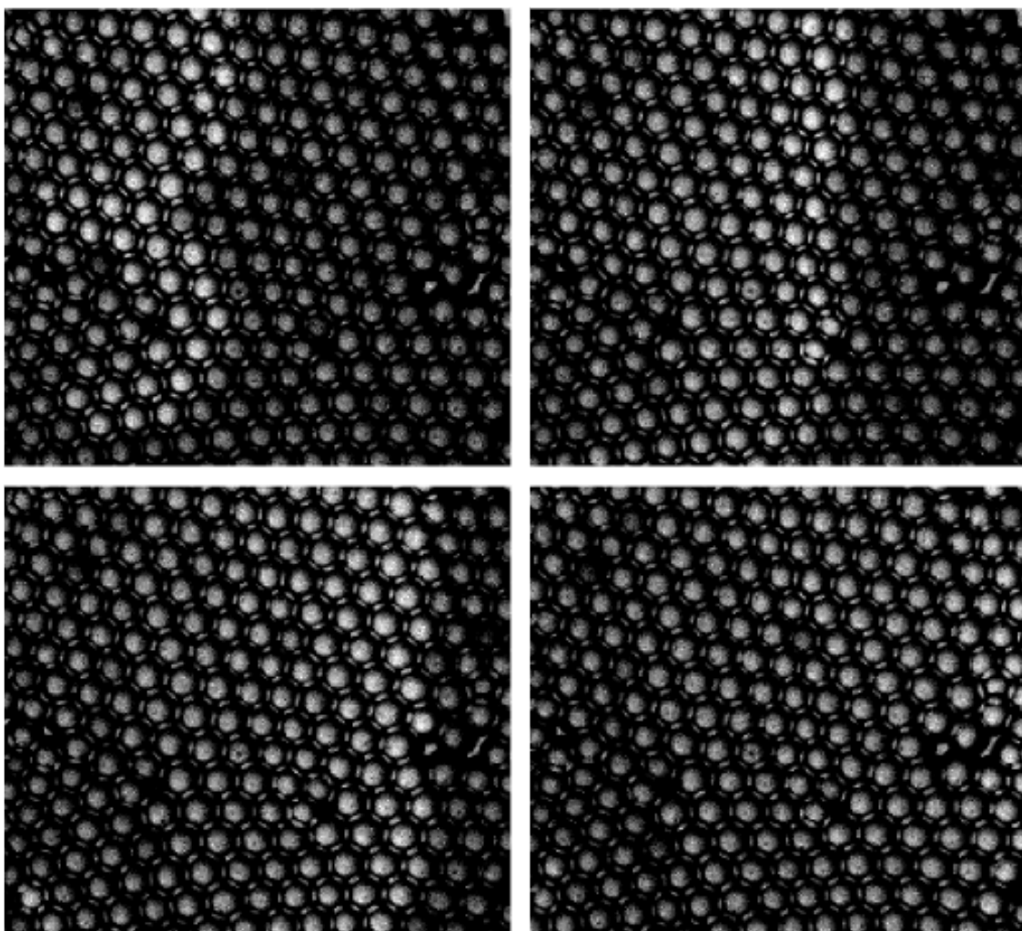
Figure 4.6: The formation of travelling waves when bilayer membranes are formed between oscillator droplets. Each image is 5 seconds apart. The droplet diameter is 30 microns.
