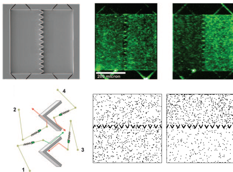
Figure 6.9: Bacterial rectification using asymmetric walls 191 . Top: A microfabricated chamber with inlet and outlet ports at top and bottom. A row of V-shaped walls divides the chamber into two halves. A fluorescence image of bacteria in the chamber where there is a uniform distribution at the start of the experiment (left) and the steady state after 80 minutes (right). Bottom (left): Schematic drawing of the interaction of bacteria with the walls. Bacteria on the left side may (trace 1) or may not (trace 2) get through the gap, depending on the angle of attack. On the right, all bacteria colliding with the wall are diverted away from the gap. Bottom (right): Snapshots from a simulation 192 , mimicking the above experiment, with point particles that move ballistically along walls.
