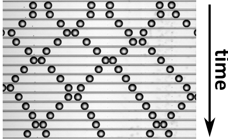
Figure 6.11: A time lapse series of droplets confined to motion in a single dimension in a microchannel. Droplets retrace their paths at each collision, reminiscent of single file diffusion.
