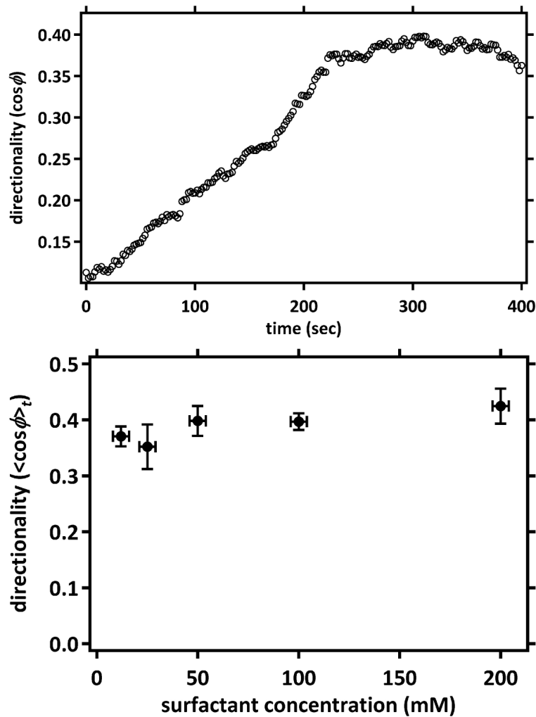
Figure 5.10: Swimmer directionality. Top: The time varying directionality is plotted for a surfactant concentration of 100 mM. A linear increase is followed by a saturation of the directionality at \sim 0.4 . Bottom: The time averaged directionality as a function of surfactant concentration, where each point is an average of \sim 50 different squirmer droplets each of diameter \sim 80 microns.
