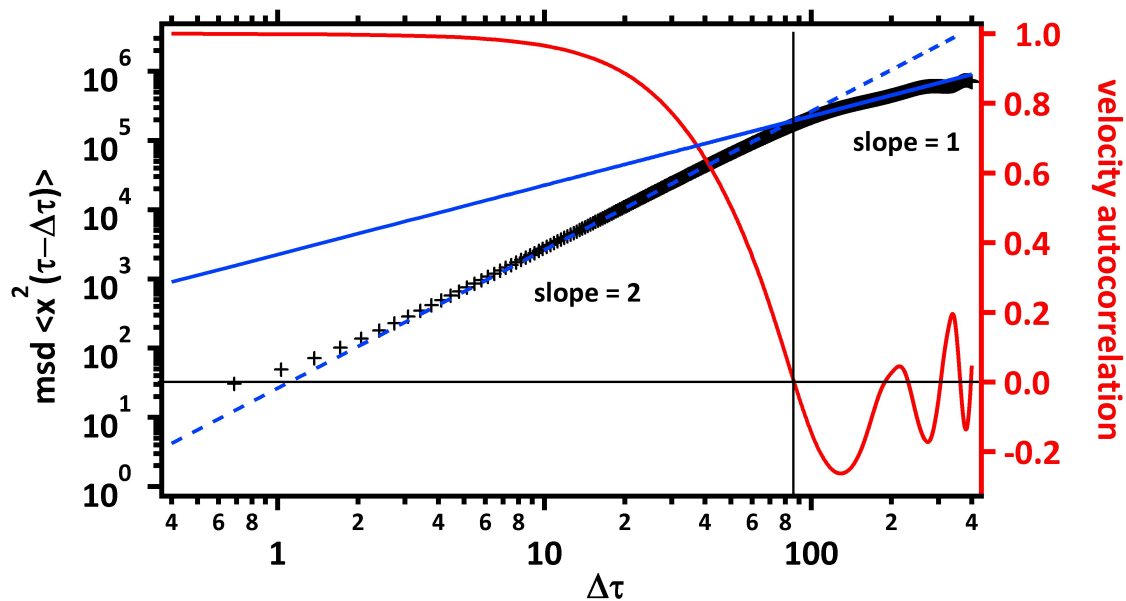
Figure 6.16: The ensemble average (of 7 droplets) of the mean square displacement as a function of time. The solid blue line is a linear fit used to calculate the effective diffusivity of the droplets. The dotted blue line has a slope of 2. The black cross-lines are a guide to identify the cross-over from the ballistic to diffusive regimes. The red trace with the axis on the right is the autocorrelation of the velocity.
