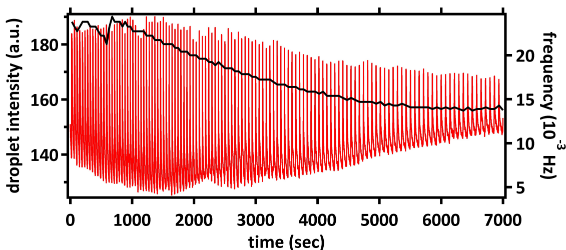
Figure 4.4: BZ oscillations in a closed reactor. The oscillation trace and its corresponding frequency (black) are plotted as a function of time.
