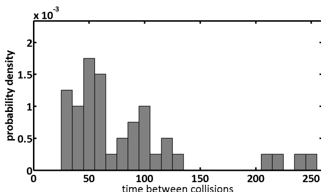
Figure 6.13: Probability density of the time between the droplet collisions.
