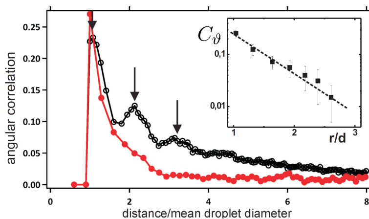
Figure 6.2: Orientational correlation
