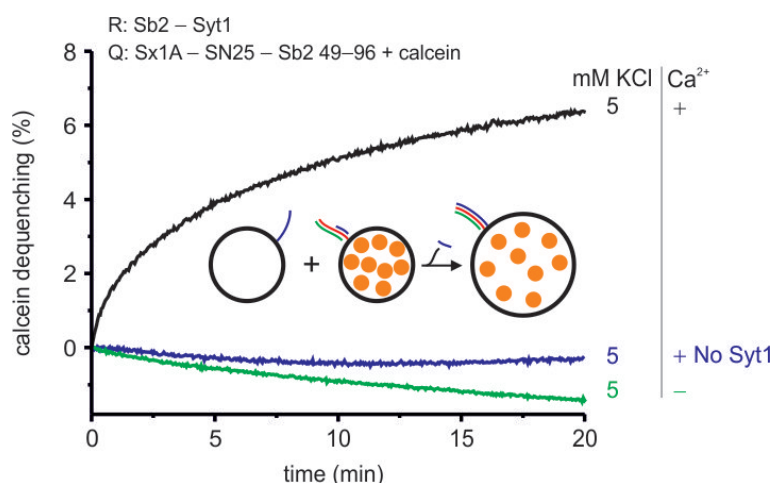
Figure 2.11: Fluorescence quenching of calcein is used to assay content mixing to confirm liposome fusion triggered by Ca^{2+} -synaptotagmin-1.
