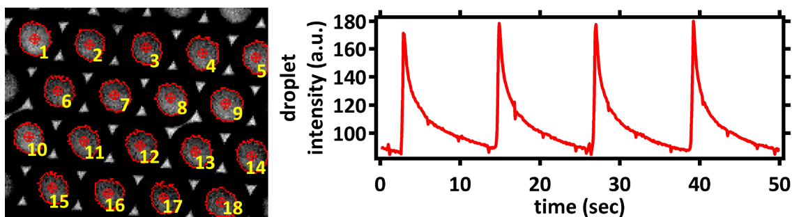
Figure 4.3: Image processing to identify the droplet oscillators and record their dynamics.
