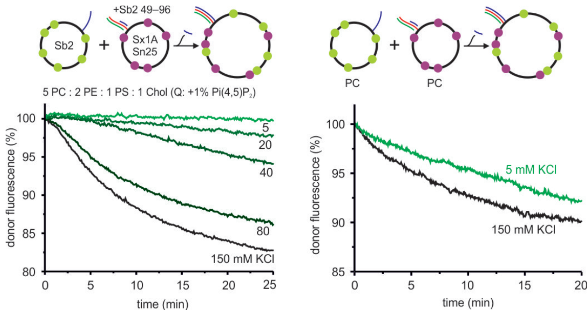
Figure 2.7: SNARE mediated membrane fusion is blocked at low ionic buffer strengths due to repulsion between charged lipids comprising the liposomes. Left panel: Liposomes contain charged lipids PS and \text{Pi}(4,5)\text{P}_2 . With the progressive reduction of the salt (KCl) concentration in the buffer solution, the fusion is reduced, until it is almost completely blocked at a concentration of 5 mM KCl (low ionic strength). The experimental conditions are shown on the top. Right panel: When only uncharged lipids are used, the fusion proceed normally even when charges are not screened at low ionic strengths of the buffer solution. The reduced kinetics at 5 mM KCl concentration is due to the increased viscosity of the buffer as described in the main text.
