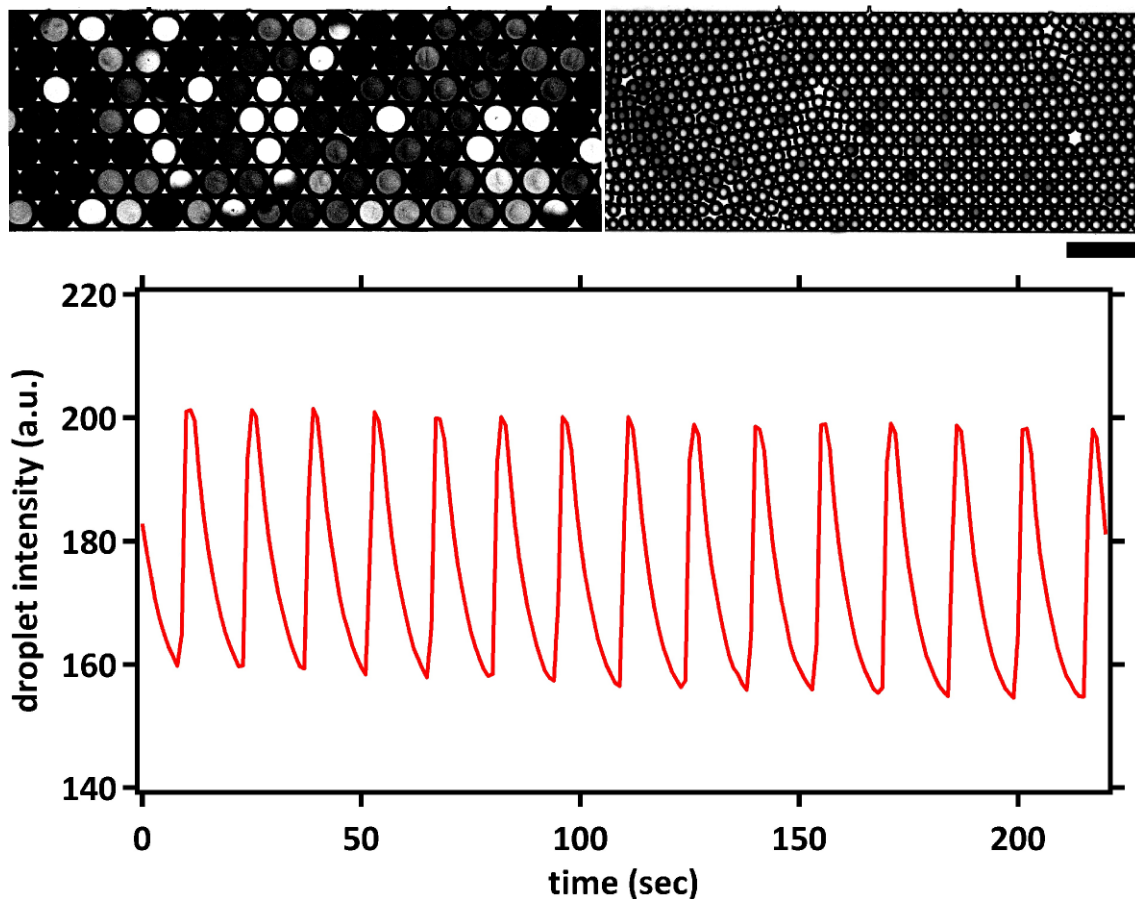
Figure 4.5: Droplet oscillators in a hexagonal packing geometry within a PDMS microchannel. Top: The different intensities of the droplets show the different BZ reaction states within each droplet for two different droplet sizes. Each droplet acts like an isolated individual oscillator without any coupling with its neighbours. Image contrast is enhanced for better visualization. Scale bar is 150 microns. Bottom: The intensity trace for a single droplet is shown as a function of time. The constancy of the frequency and amplitude of the oscillations can be clearly seen.
