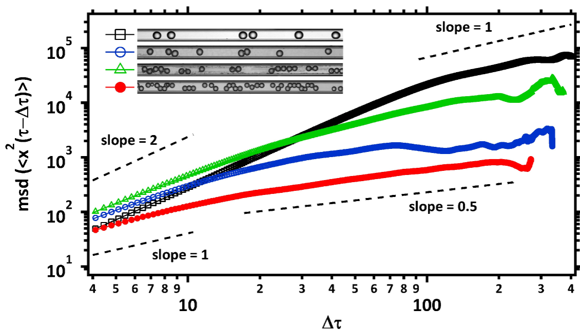
Figure 6.17: Ensemble averaged MSDs for different confinements of droplets as shown in the inset of the legend.
