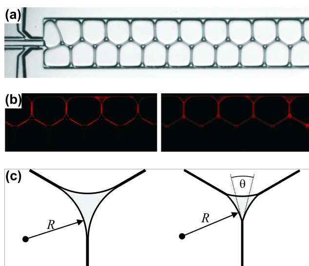
Figure 1.5: (a) Gel emulsion in a channel ( 500\ \mu\text{m} wide) at very low volume fraction of the continuous oil phase (below 10%). (b) Micrograph of an emulsion like the one shown in (a), taken at the fluorescence wavelength of the dye (di-4-anepps) which was fed into the upper row of droplets. Illumination is by UV light. Left: as prepared. Right: a few seconds later, when membranes have formed. (c) Geometry of Plateau borders, where three oil lamellae (or membranes) meet at 120 degrees. Left: as prepared. The droplet surfaces meet tangentially. Right: after membranes have formed. The contact angle, \theta , at the end of each membrane has attained a finite value.
