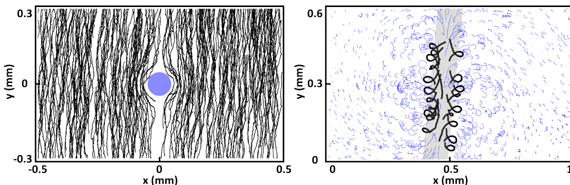
Figure 6.5: Trajectories of tracer particles around a single droplet squirmer over a 16 s duration Left: in the co-moving reference frame of the squirmer (shown as blue circle, which represents the approximate size of the actual droplet) and Right: in the laboratory frame of reference. The grey box indicates the approximate path of the squirmer. The closed loops of the tracer tracks (black) are seen close to the swimmer path.
