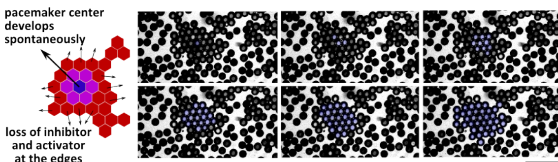
Figure 4.9: Formation of a target pattern in a 'island' or 'peninsula' type of droplet network. Left: A schematic of a hexagonal arrangement of droplets which form an 'island'. At the outer edges of the structure, the excitatory and the inhibitory components are lost to the oil phase (shown by the arrows), while in the center, they are concentrated leading to the formation of pacemaker center. Right: A target pattern develops within a 'peninsula' of droplet oscillators. The excitation and wave pattern are shown in blue for easy visualization. The scale bar is 500 microns.
