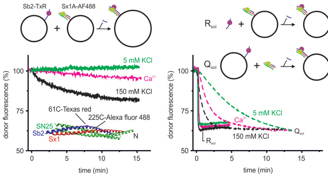
Figure 2.8: SNARE nucleation is blocked at low ionic buffer strengths. Left panel: When the fluorescently labelled SNARE proteins are present in their respective liposomes, reducing the ionic strength leads to a complete blocking of SNARE nucleation. The addition of 1 mM Ca^{2+} does not change the situation. Right panel: In the absence of the repulsive interactions caused due to the lipids in the liposomes, SNARE nucleation proceeds normally irrespective of the ionic strength of the buffer used.
