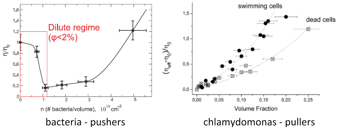
Figure 6.18: Rheological measurements on Left: Bacterial suspensions which are pusher type swimmers 196 and Right: Chlamydomonas suspensions which are puller type swimmers 197
