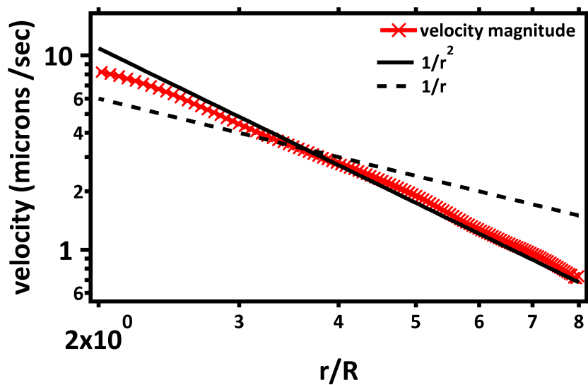
Figure 5.6: The fluid velocity calculated at the equator of the swimming droplet. It shows a decay of \sim 1/r^2 as the distance from the droplet increases.
