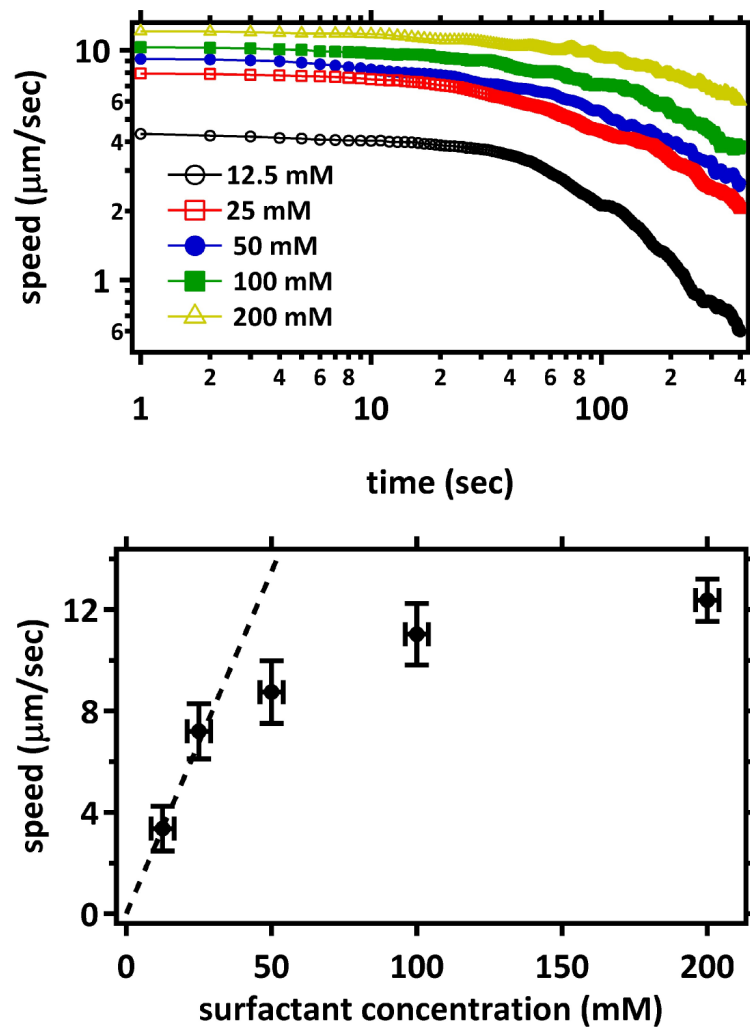
Figure 5.7: Top: Swimmer speed as a function of time, at different surfactant concentrations, where each curve is an average of \sim 50 different squirmer droplets each of diameter \sim 80 microns and Bottom: The initial swimmer speed (average of first 40 time points) as a function of surfactant concentration
