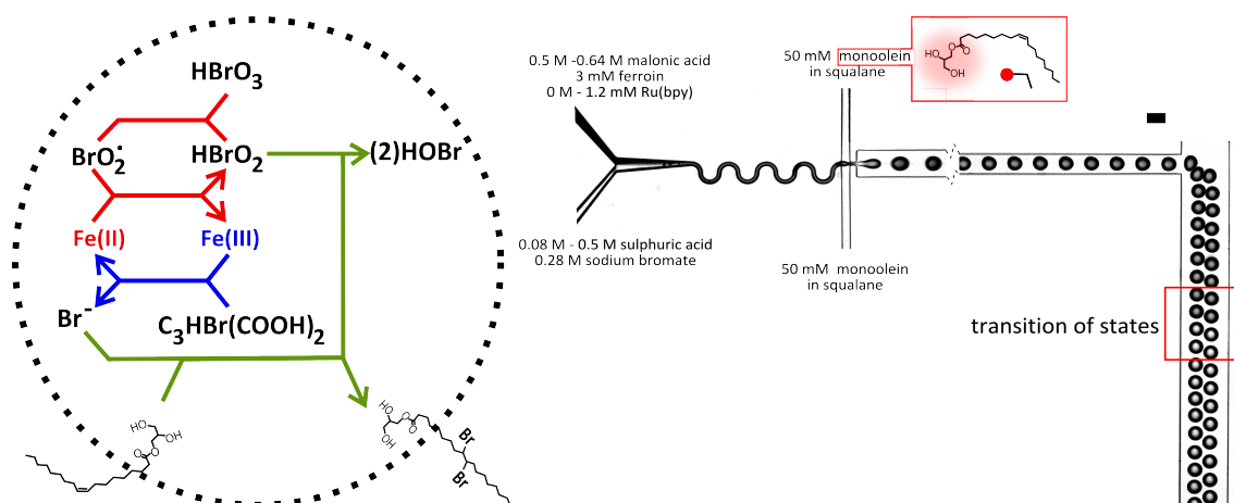
Figure 4.1: Production of monodisperse oscillator droplets. Left: The BZ reaction consists of two loops (i) an autocatalytic and (ii) an inhibitory cycle. The reaction state can be visualised by the colour of the ferroin catalyst. In our setting, an additional reaction with the unsaturated mono-olein surfactant occurs as shown. Right: The contents of the BZ reaction are mixed on the microfluidic chip to prevent any pre-reaction. Seen through an optical 480/20 nm notch filter, the transition from red colour to the blue colour of the BZ reaction is seen by the change in the brightness of the droplet.
