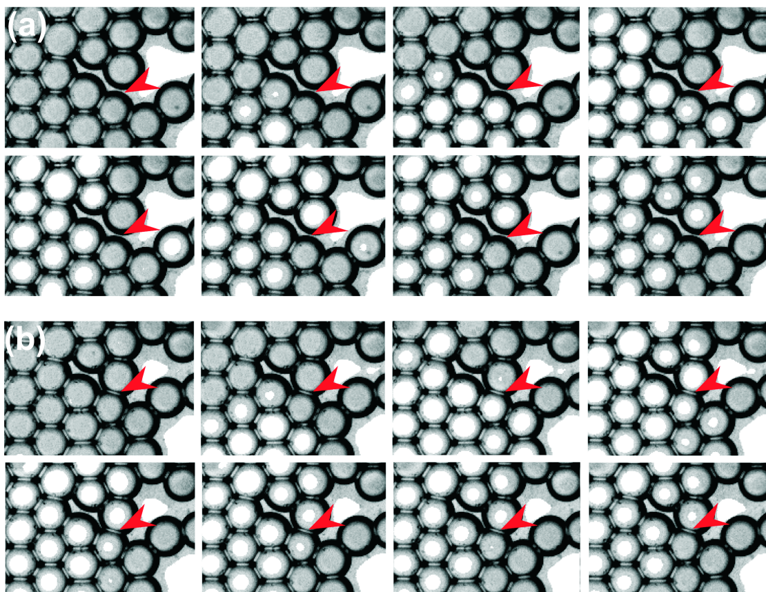
Figure 4.7: Demonstration of the influence of membrane coupling on an excitation wave in a larger raft of droplets. The oil phase consists of squalane with 50 mM/l mono-olein. The aqueous phase is 0.5 M sulphuric acid, 280 mM sodium bromate, 0.5 M malonic acid, and 3 mM ferroin. (a) The droplet surfaces indicated by the red arrow are very close, but there has yet no membrane been formed. The excitation wave (coming from below) passes around the arrow, the excitation does not directly cross the gap between the two droplets. (b) After the membrane has formed, the excitation wave passes through the site indicated by the arrow.
