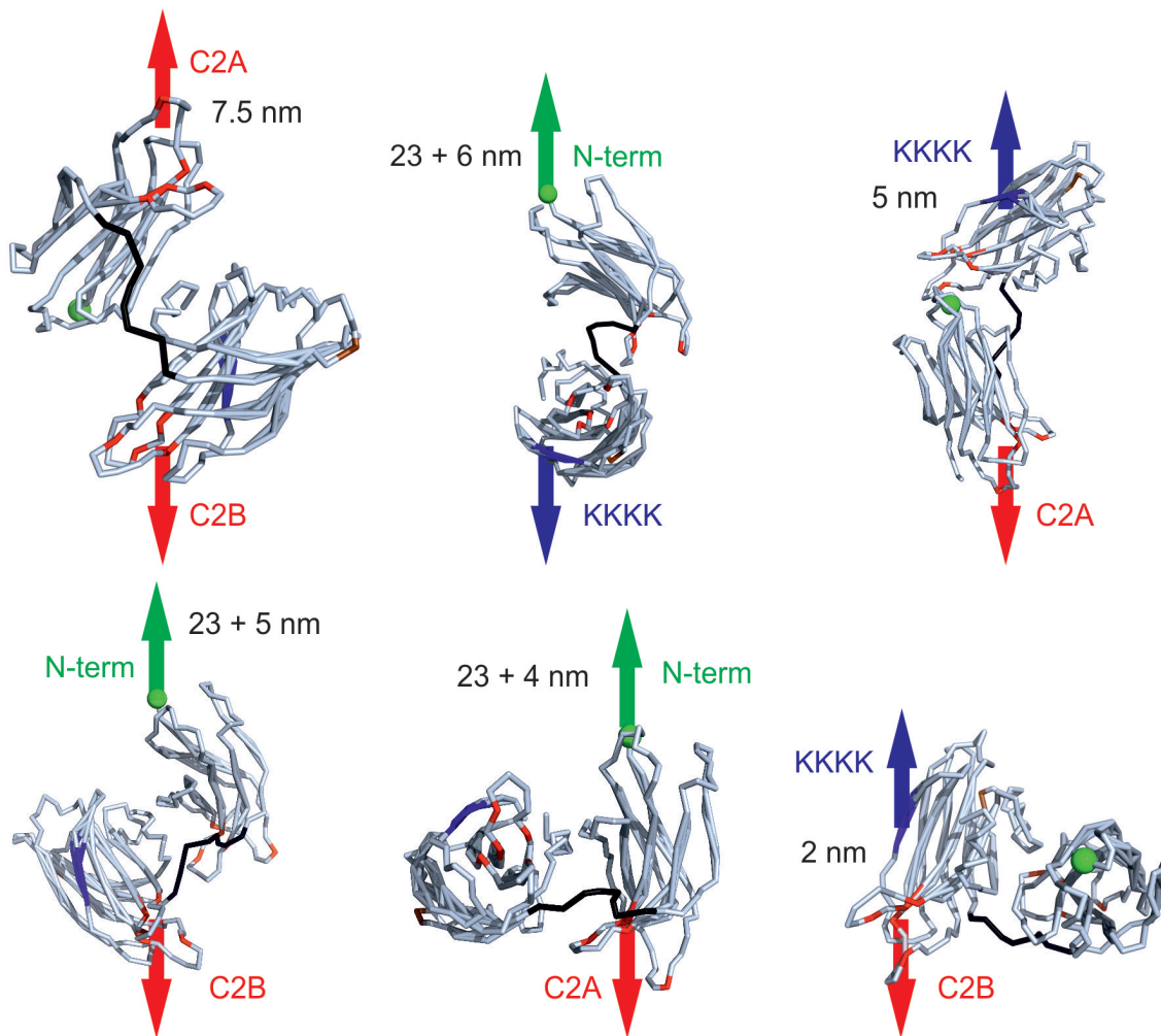
Figure 2.13: Molecular dynamic simulations to estimate the maximal distances between the various domains. In the simulations, we pulled pair-wise on various membrane binding sites of the C2AB-domain: the N-terminus (green), the polybasic lysine patch (blue; KKKK) and the Ca^{2+} -binding sites of the C2A- and C2B-domain (red). The two conserved arginines (R398 and R388) are shown in brown; the linker is in black. The N-terminus is connected to the transmembrane helix with a 61 residue linker that can extend to \sim 23 nm. Maximal distances are indicated in the figure; these are an approximate for the tethering distances of the membranes, but do not take into account additional interactions such as membrane insertion and bending.
