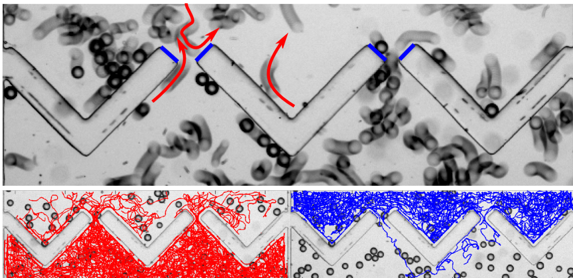
Figure 6.10: Rectification of droplet squirmers by spatial asymmetry. A 2-dimensional chamber is separated by V-shaped walls with gaps of 75 microns between them. The mean droplet size is 50 microns. Top: A time lapse image showing typical squirmer interactions with walls. Droplet in the bottom half of the chamber are guided through the gaps, while those that start at the top bounce back from the walls, leading to an effective rectification. Bottom: Squirmer trajectories over a duration of 10 minutes are overlaid on the image. Red trajectories are for those droplets which were in the bottom half of the chamber at the start of the experiment. Similarly blue trajectories represent droplet that started in the top half. The rectification effect can be seen by the number of the red trajectories that go through to the other side compared with the blue ones.
