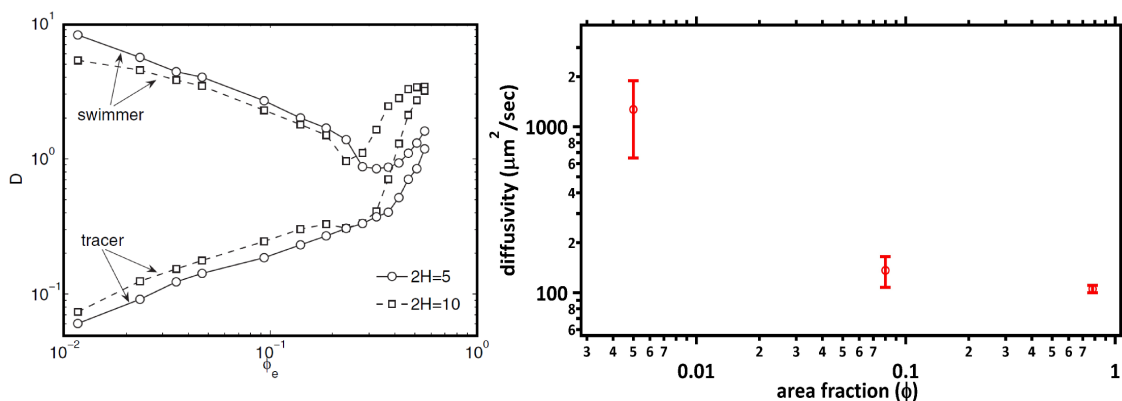
Figure 6.4: Diffusivity as a function of area fraction. Left: Results from a simulation done by Hernandez et. al. 173 Right: Diffusivities calculated from the long time statistics of the MSD plots shown in Fig. 6.3.
