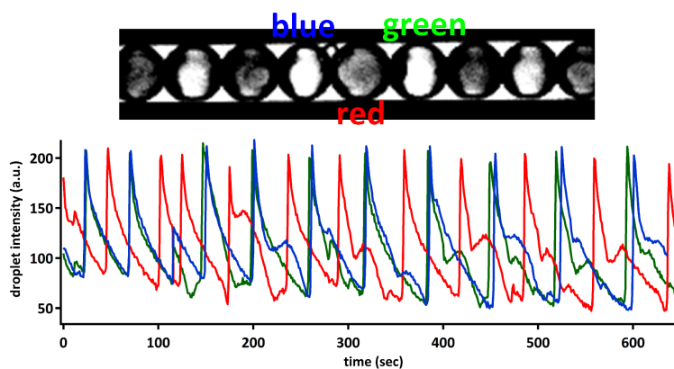
Figure 4.13: Antiphase pattern in a 1 dimensional oscillator network. Top: Droplet oscillators in a glass microcapillary. Each droplet pair is connected by bilayer membranes. The droplet diameter is 100 microns Bottom: Time trace of the droplet oscillations shown for the three droplets in the center of the top image. The red, blue and green traces correspond to the droplets marked as shown.
