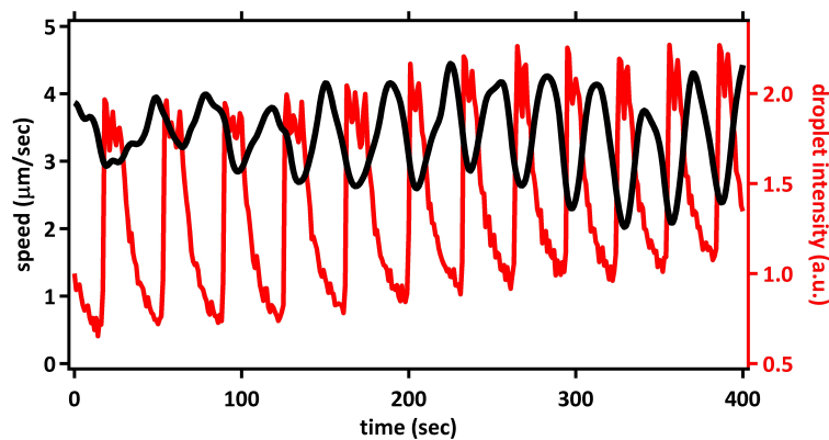
Figure 5.9: The velocity as a function of time for an squirmers when an oscillating chemical reaction (BZ) takes place in the droplet. The optical transmission of the droplet is plotted in red (arbitrary units, linear scale) along with the velocity trace.
