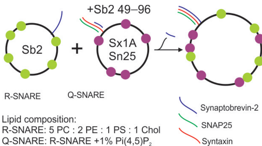
Figure 2.3: The cartoon sketch above indicates the liposomes conditions used in the experiment. Large black circles indicate the liposomes. Sb2 stands for Synaptobrevin2, Sx1A is Syntaxin 1A and Sn25 is SNAP25. The green and purple dots indicate the green donor fluorophore and the red acceptor fluorophore, of the FRET pair, respectively. A tiny fragment (residues 49-96) of synaptobrevin-2 is added to the Q-SNAREs to prevent spontaneous fusion. Fusion is then triggered by cleaving this fragment from the Q-SNAREs by the addition of an appropriate enzyme. The lipids and their ratio used in the preparation of the liposomes are shown below. PC, PS, and PE are abbreviations for the lipid head groups. PC: Phosphatidylcholine, PS: Phosphatidylserine and PE: Phosphatidylethanolamine, Chol: cholesterol.
