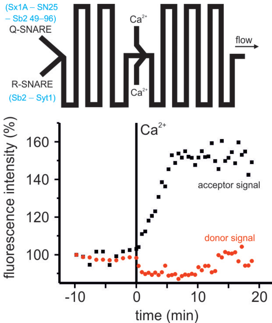
Figure 2.9: Microfluidic triggering of membrane fusion at low ionic strengths by mediating Ca^{2+} -synaptotagmin-1 interactions. Top panel: The channel geometry to study the Ca^{2+} triggering. The Q-SNARE and the R-SNARE are initially mixed and their fusion kinetics can be followed by taking images at multiple turn segments. After a certain time, Ca^{2+} is introduced from a side channel from which point on, the Ca^{2+} triggered fusion kinetics can be studied. Bottom panel: The fluorescence intensities of the donor and acceptor fluorophore are shown as a function of time. The time point of Ca^{2+} addition is taken as t = 0 . Before the addition of Ca^{2+} no fusion takes place in spite of the synaptotagmin-1 already present in the R-SNAREs. As soon as Ca^{2+} is added, fusion increases dramatically.
