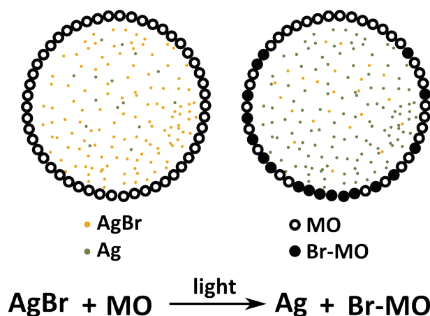
Figure 5.11: Scheme for light controlled release of bromine. Silver bromide colloids are included in the aqueous phase which are degenerated by light to release bromine, which participates in the reaction with pristine mono-olein.
