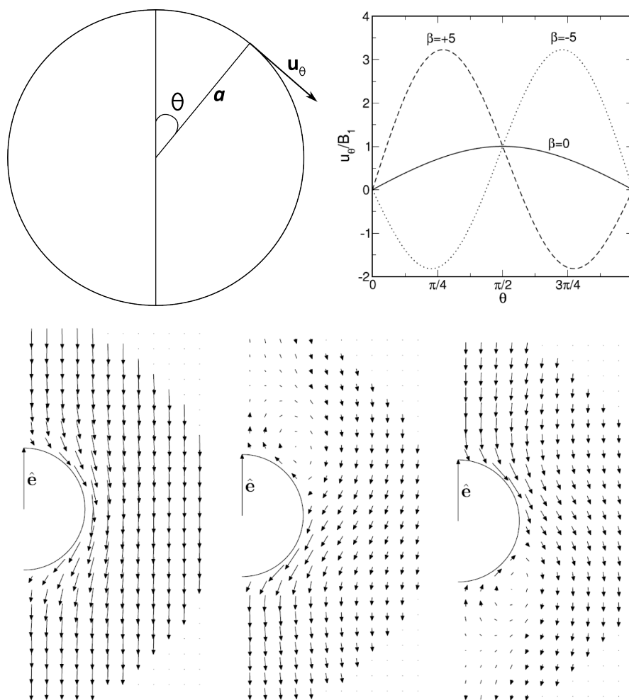
Figure 5.4: A model squirmer. Top(left): A schematic of an axisymmetric surface velocity u_\theta = B_1 \sin\theta + B_2/2\sin 2\theta on a sphere. Top(right): The surface velocity at different relative strengths of the spherical harmonic modes and (Bottom): their corresponding flow fields. \beta = 0 corresponds to a neutral squirmer and \beta < 0 is a pusher and \beta > 0 is a puller.
