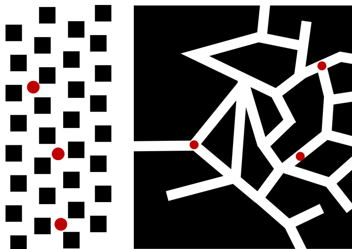
Figure 6.19: Droplet swimmers on 2-D lattice and random network topologies. White spaces represent 'channels', black regions are walls and the red circles indicate swimmers.
