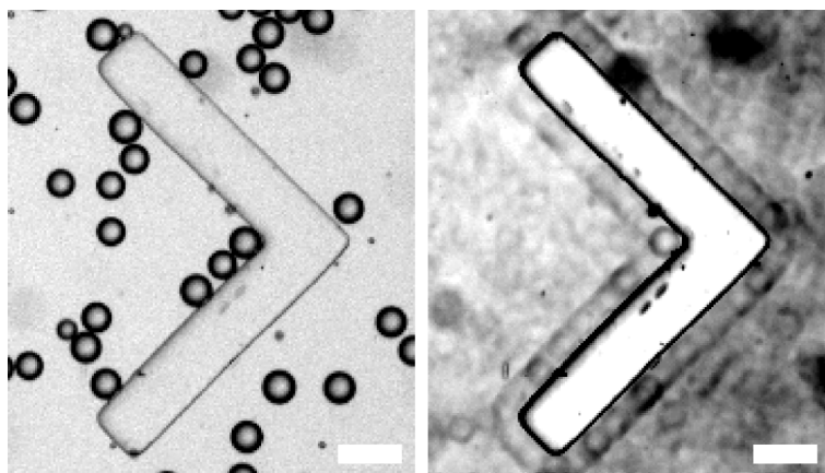
Figure 6.8: Squirmers at angular walls. Left: Squirmers are observed in a 2 dimensional space with a V-shape wall made from PDMS in the middle. Right: An overlay of 600 images shows an aggregation near the wall, in particular as a monolayer. The contrast of the image has been enhanced for improve visualisation. Scale bar: 100 microns
