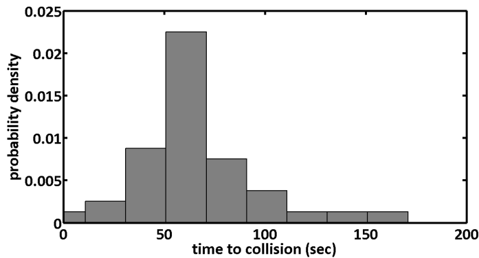
Figure 6.15: Frequency distribution of the rescaled time between the droplet collisions.
