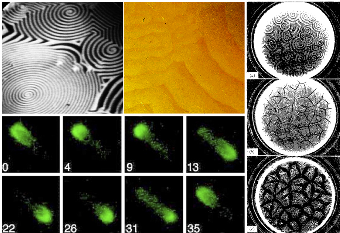
Figure III.1: Clockwise from top left : Spatiotemporal patterns such as spirals and traveling waves in catalytic reactions, the Belousov-Zhabotinsky reaction, aggregating social amoeba and Min-oscillations in bacteria. (Images taken from 126,127 )
