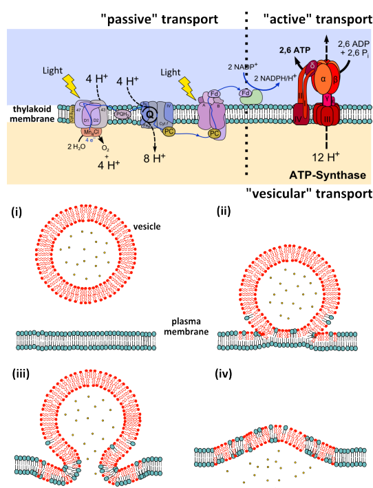
Figure II.1: Passive, active and vesicular traffic across membranes. Top: Schematic of electron and proton transport in photosynthesis. Bottom: Biomolecular cargo delivery via (i) fusion of bilayer membranes, which proceeds through various stages such as (ii) docking (iii) pore (stalk) formation and finally (iv) full fusion.
