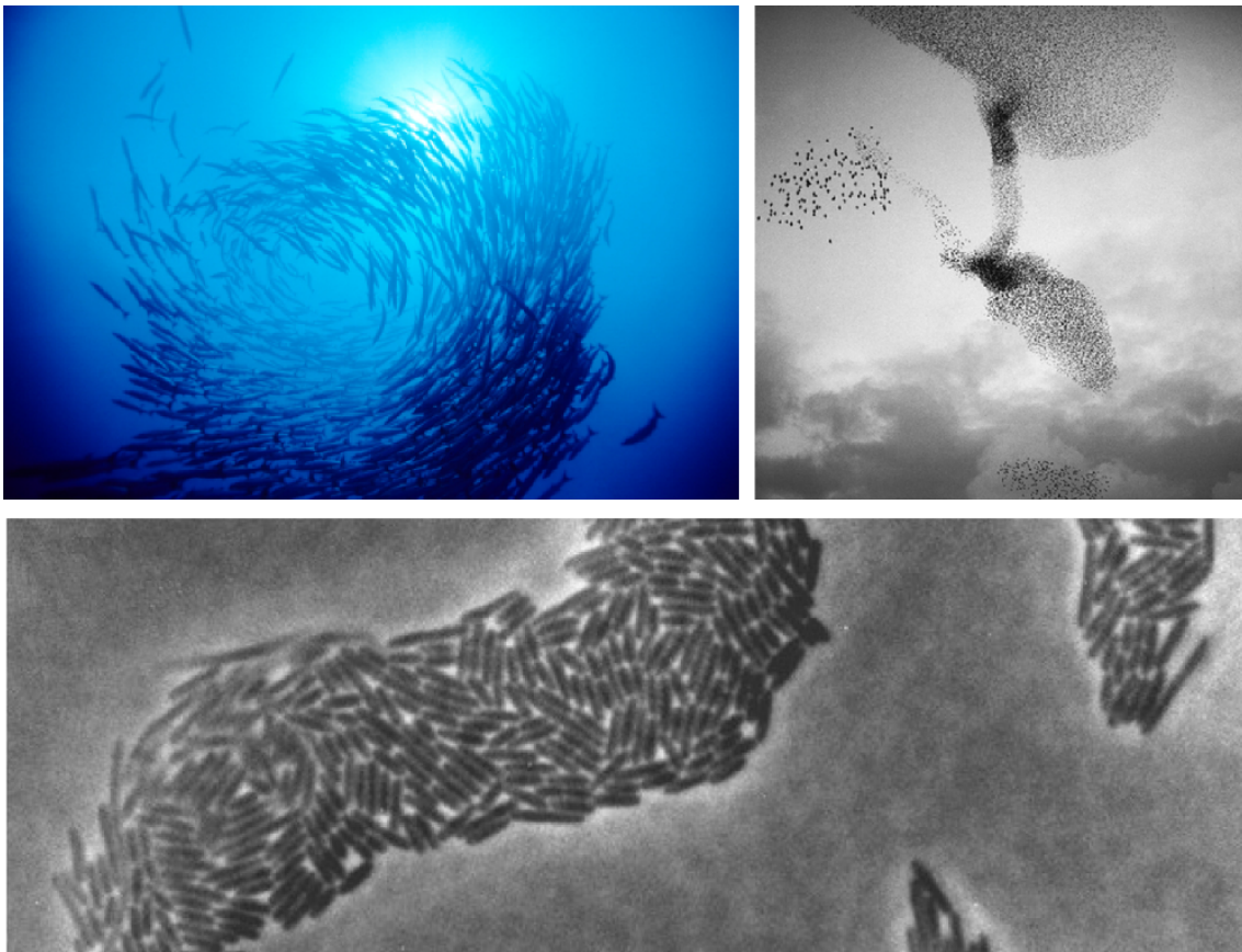
Figure III.2: Pattern formation at various scales due to flocking of swimming fish schools, flying starlet populations and gliding bacteria. (Images taken from 128–130 )
