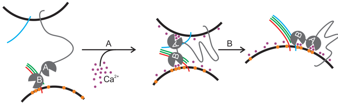
Figure 2.14: Model for synaptotagmin-1 mediated lipid mixing. In the absence of Ca^{2+} , synaptotagmin-1 (grey) tethers to anionic membranes, and particularly to Pi(4,5)P_2 (orange) via its polybasic lysine patch. The distance is too far for SNARE formation to occur (synaptobrevin-2: blue; Syntaxin-1A: red; SNAP-25: green). (Step A) In the presence of Ca^{2+} (purple), a transitional conformation change occurs and synaptotagmin-1 binds the membrane via its calcium binding pockets and basic residues on the C2AB-domain. This drives the membranes together and SNARE complex formation can occur. (Step B) The SNARE complex formation drives membrane fusion.
