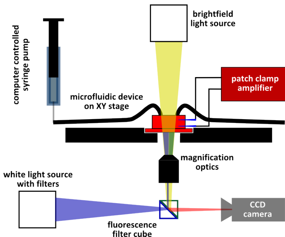
Figure 1.2: A patch clamp amplifier is integrated to a microfluidics station on inverted microscope to make electrical recordings in microfluidic devices
