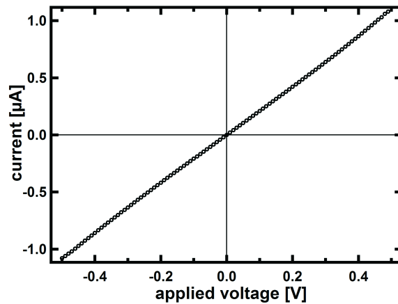
Figure 1.11: Current/voltage characteristic of a mono-olein membrane doped with Gramicidin A ion pores.
