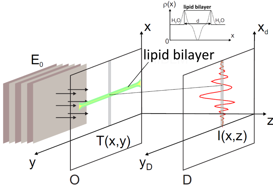
Figure 3.3: The mfBLM at position O is described by a transmission function T(x,y) obtained by projection of the electron density \rho(x) along the z -axis. After free space propagation of the exit wave over a distance z along the optical axis, a Fresnel interference pattern I(x) is recorded in the detector plane D , representing a phase contrast image of the projected density profile.
