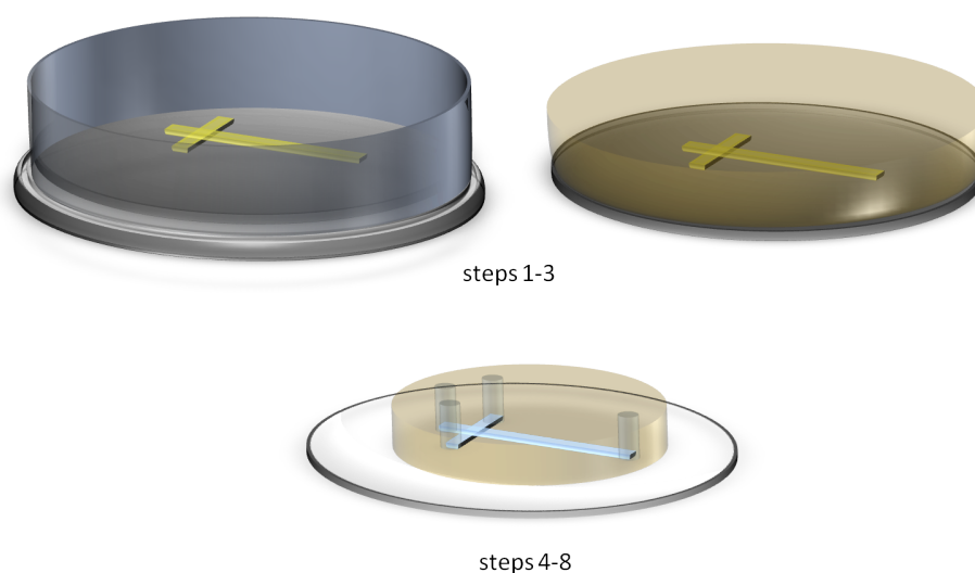
Figure A.2: Soft lithography technique for the preparation of PDMS microfluidic devices.
