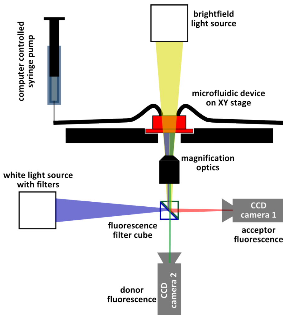
Figure 2.4: Experimental setup for performing microfluidic FRET experiments to study membrane fusion. A microfluidic device made using PDMS soft lithography is mounted on an inverted microscope. The flow through the device is regulated by computer controlled syringe pumps. The FRET fluorescence is recorded on two separate CCD cameras, one for the donor and the other for the acceptor fluorescence wavelengths respectively. The donor fluorescence is excited by using filtered light from a white light source.
