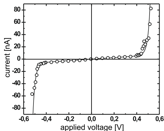
Figure 1.12: Current/voltage characteristic of a mono-olein membrane. Aside from an ohmic central part, there is a pronounced rise in the current at a threshold voltage of about 500 mV. This is attributed to reversible electroporation. The solid curve corresponds to what would be expected theoretically in that case.
