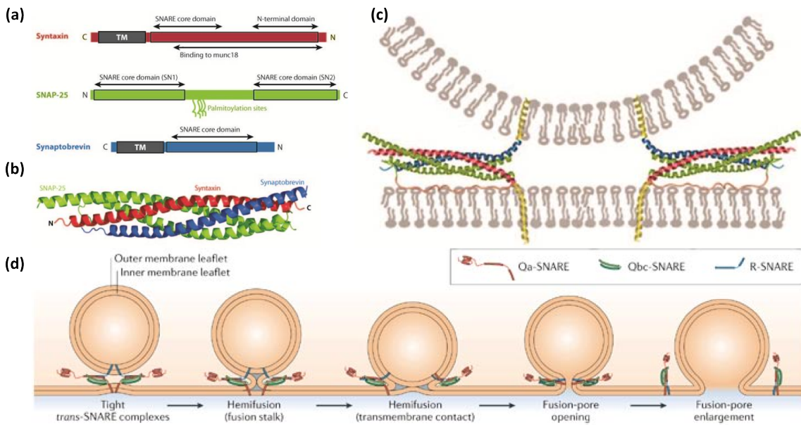
Figure 2.1: SNARE protein complex and SNARE-mediated membrane fusion. (a) Schematic of the 3 components of the SNARE complex: Syntaxin, SNAP-25 and Synaptobrevin. Syntaxin and Synaptobrevin have transmembrane domains (TM) at their C terminals. The TM domains embed into the lipid bilayer. SNAP-25 and Syntaxin are present on the plasma membrane. Synaptobrevin is present on the vesicle. (b) The coil-coil structure of the SNARE proteins. The coiling proceeds from the C terminals towards the N terminals. (c) When the proteins coil, the two lipid bilayers of the plasma membrane and the synaptic vesicle are pulled close together (d) Once the membranes are close enough, the lipid bilayers fuse through a sequence of events such as hemifusion, formation of a fusion pore and finally complete fusion. (Figures reproduced with permission from 20 and 19 )
