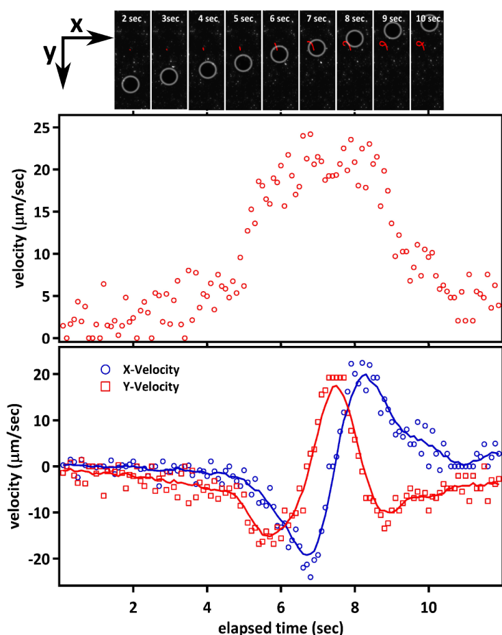
Figure 6.6: Dynamics of closed loop formation. Top: Snapshots from an experiment showing the motion of the squirmer droplet (white circle) with fluorescent tracers (white spots) around. The trajectory of a single tracer which forms a closed loop is shown in red. Middle: The corresponding velocity of tracer as a function of time. Bottom: The X and Y components of the tracer velocity.
