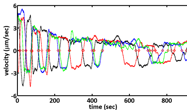
Figure 6.12: Velocity of droplets in a channel as a function of time, shown for 4 representative droplets. The traces are coloured for distinguishability. The red circles mark the zero crossings of the velocity traces, indicating droplet collisions.
