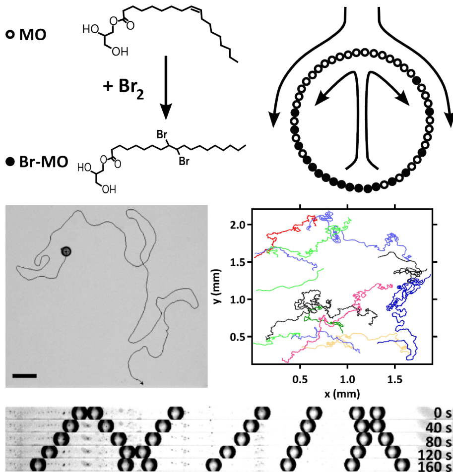
Figure 5.3: Top: Schematic of a micro-droplet squirmer. Bromination increases the tension of the droplet surface from 1.8 mN/m to 3.1 mN/m. The convective flow pattern (shown in the rest frame of the droplet) is accompanied by a gradient in the bromination density. The corresponding Marangoni stress propels the droplet. Middle(left): Path of a single squirmer droplet. The persistence length is clearly large compared to the droplet radius, indicating propelled motion (Scale bar: 300 microns). Middle (right): Droplet trajectories over an interval of \sim 90 s. Bottom: Time lapse series of seven droplets in a microchannel. The droplets change direction without noticeable reduction in velocity.
