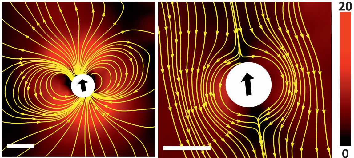
Figure 5.5: Velocity field around a droplet squirmer. The flow velocity and streamlines in Left: the reference frame of the laboratory and Right: the co-moving frame of reference. The magnitude of the flow velocity (color code) and streamlines are along a horizontal section through the center of a squirmer droplet. Scale bar: 100 microns; velocity scale (right) in microns per second.
