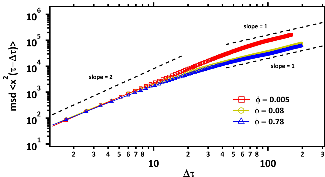
Figure 6.3: The ensemble averaged mean square displacement (MSD) for a 2- dimensional monolayer of squirmer population at different area fractions. Each population has between 50 - 500 squirmer droplets.
