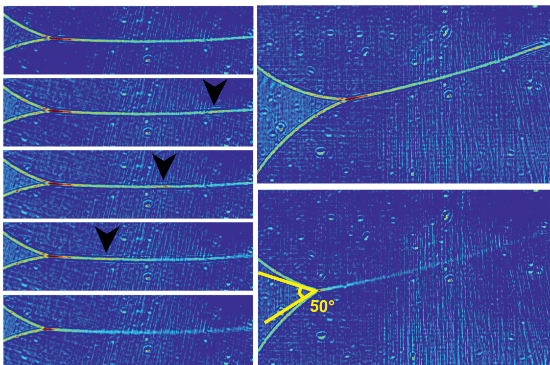
Figure 3.6: Left: Image series of the "zipper-like" effect, which occurs during the transformation from a bulk film to a bimolecular membrane from top to bottom. Right: The migration of solvent and the formation of a bilayer membrane leads to a change in the opening angle between the lipid monolayers at the start of the lipid bilayer as shown.
