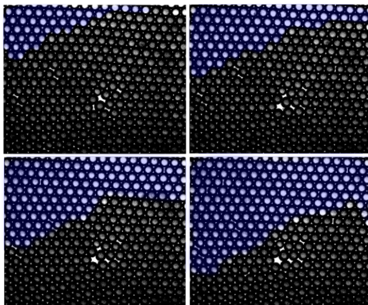
Figure 4.11: Travelling waves are formed in large densely connected oscillator networks. Each image is spaced 5 seconds apart. The excitation is coloured blue for easy visualization.
