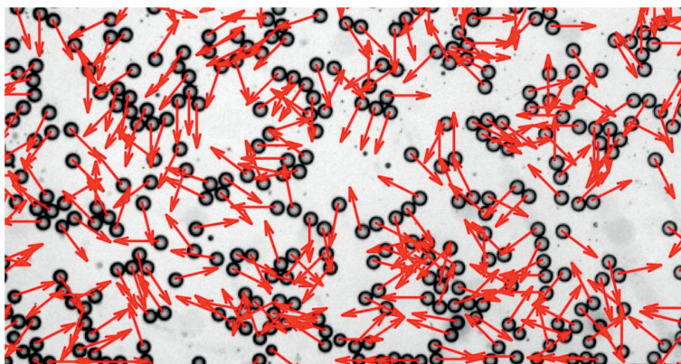
Figure 6.1: Velocity vectors overlaid on droplets
