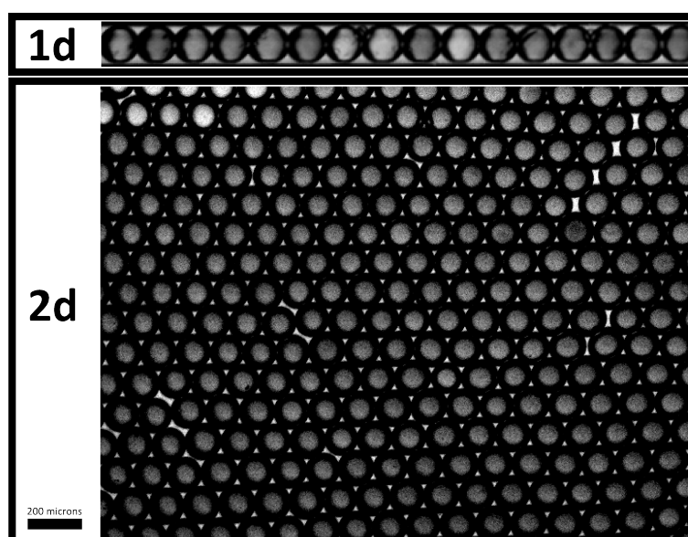
Figure 4.2: Storage of droplet oscillations in one and two dimensional confinement for observation of their dynamics.
