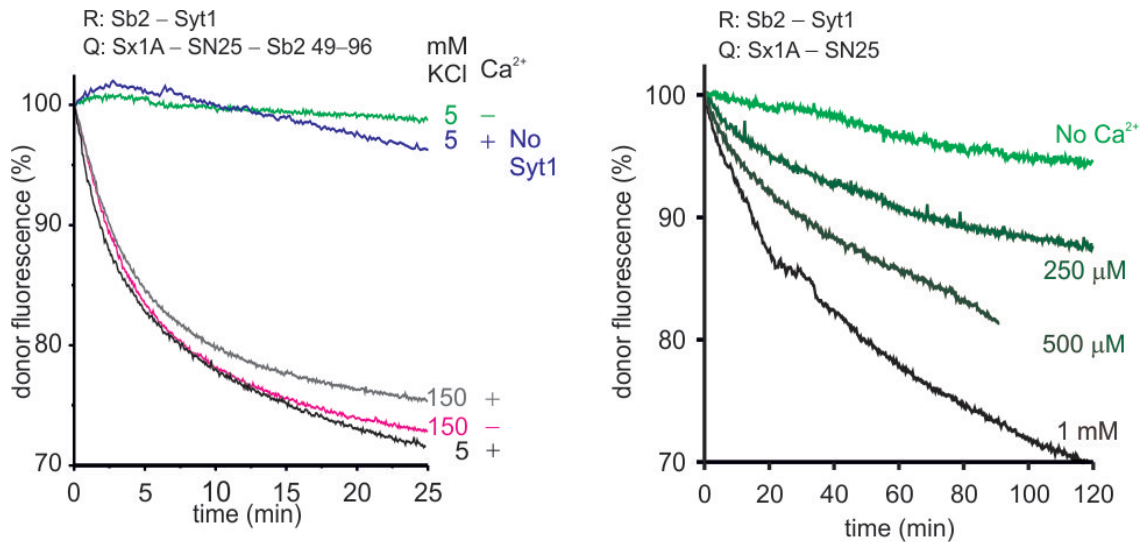
Figure 2.10: Left panel: Membrane fusion at low ionic strengths is strictly dependant on the presence of both Ca^{2+} and synaptotagmin-1. In the absence of either of these, fusion does not proceed. When both these are present, fusion proceeds normally even at low ionic strengths. At normal ionic strengths however, neither Ca^{2+} nor synaptotagmin-1 dramatically changes the kinetics. The + and - symbols indicate the presence and absence of Ca^{2+} respectively. Right panel: The fusion rate depends on Ca^{2+} concentration. A roughly linear dependance is seen.
