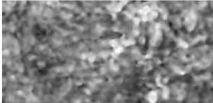
Figure 3.10: Example of a velocity map for the height of 600km; the granulation pattern is hardly visible.
