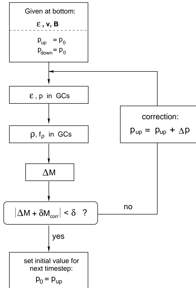
Figure 3.6: Flow diagram of the pressure adjustment procedure
