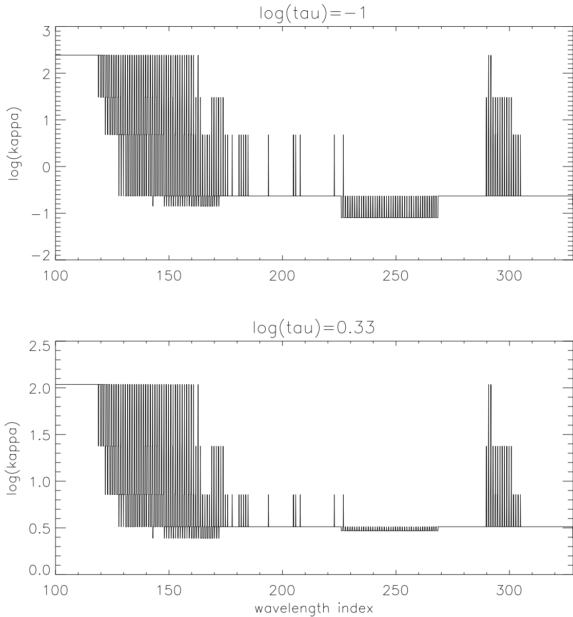
Figure 4.13: The bin-sorted opacity spectrum at two different heights for the model with split continuum. The heights correspond to optical continuum depths of \log(\tau_{5000}) = -1 and 0.33 , respectively. As a result of the sorting and averaging procedure, the opacity values that occur in these spectra form a discrete set. Note the relative change with depth of the two continuum levels in the frequency windows with indices 150 - 175 and 225 - 270 .
