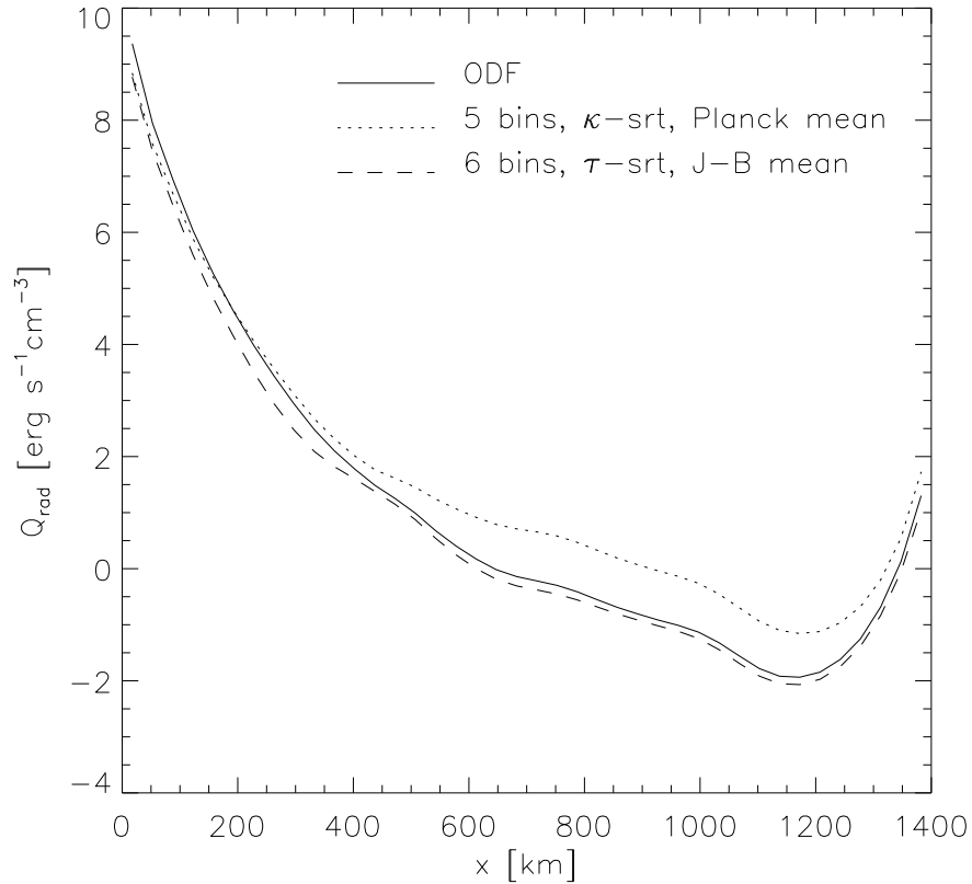
Figure 4.26: Q_{\text{rad}} for a horizontal cut through a 2D snapshot at a height of approx. 700 km above \tau_{5000} = 1 . For x > 400 km the J - B mean improves the quality of the approximation.
