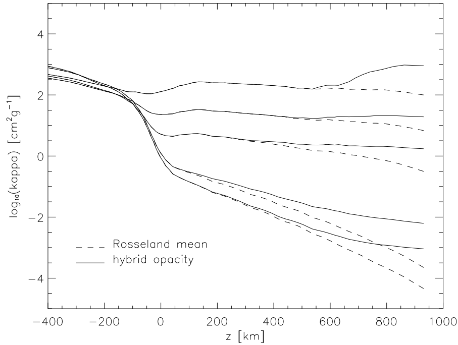
Figure 4.12: The bin-averaged opacities as a function of height for the 5 bin solution. Both the Rosseland mean and the hybrid opacity defined in Eq. (4.34) are shown. For z < 0 , the opacity values become similar for all bins, resulting in an effectively grey treatment of the radiative transfer.
