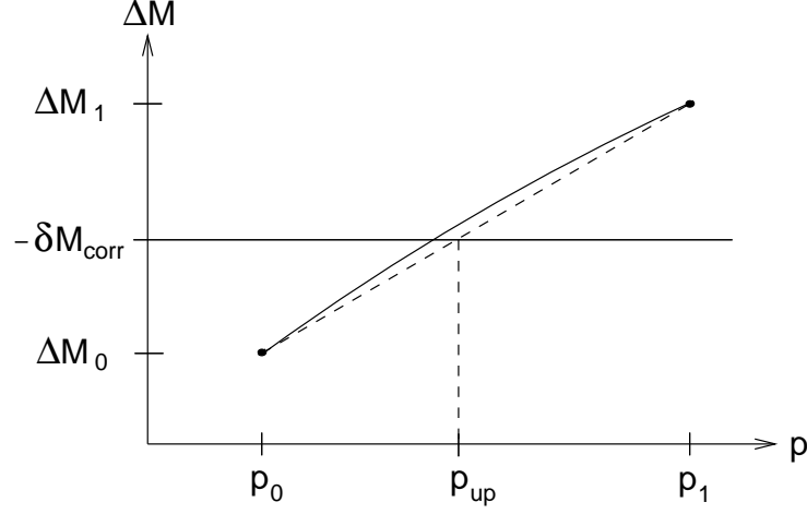
Figure 3.5: Determining the pressure correction in upflow regions with a secant method: a new value p_{\text{up}} is obtained by linear interpolation of the mass deficit function \Delta M(p) between the two previous guesses p_0 and p_1 .
