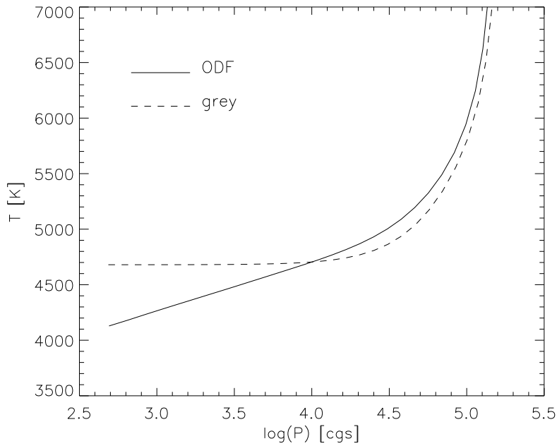
Figure 4.9: Flux-constant temperature stratifications resulting from ATLAS9, for the ODF-based solution and the grey case using the Rosseland mean opacity; the height in the atmosphere increases towards the left. The inclusion of line opacities in the ODF-solution leads to considerable cooling in the upper layers and a temperature increase below.
