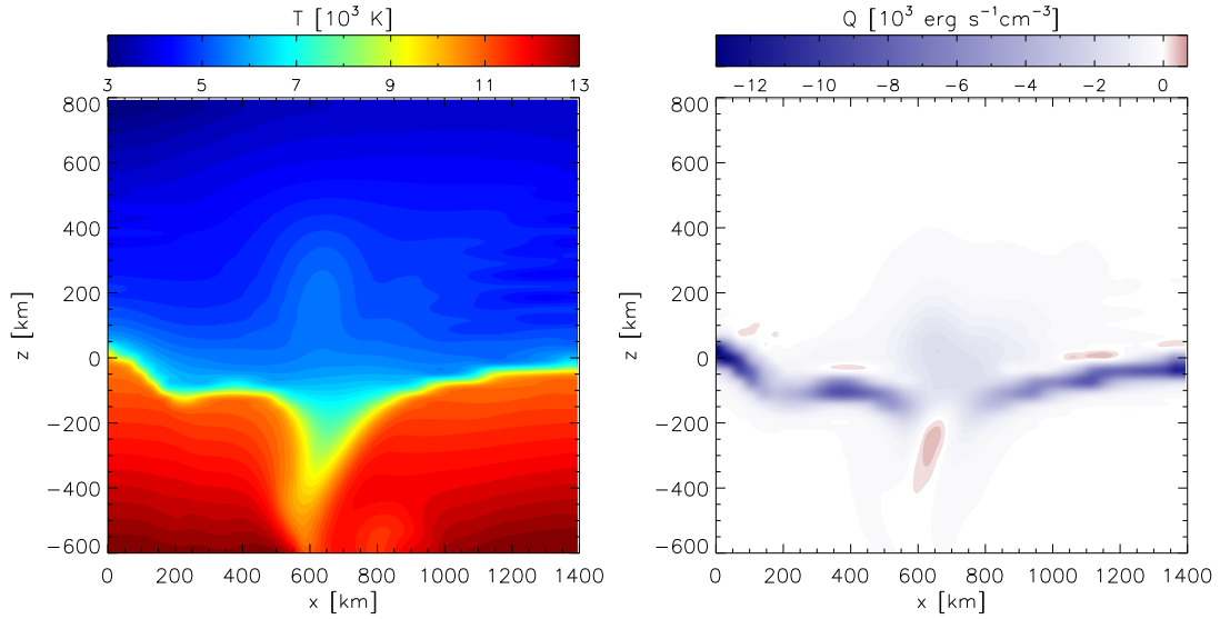
Figure 4.19: Left: Temperature plot of a 1.4 \times 1.4 \text{ Mm}^2 cut-out from a two-dimensional simulation snapshot (Ploner et al. 1999). Right: The corresponding ODF based radiative heating rate.
