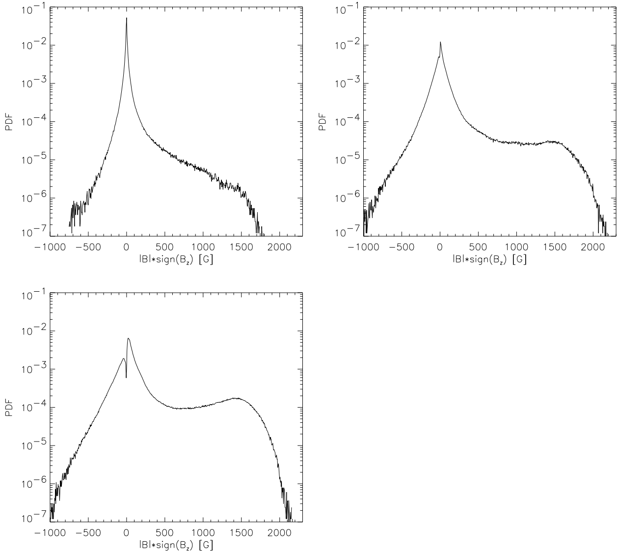
Figure 5.25: Probability distribution functions for the magnetic field, for all three magnetoconvection runs. Top left: 10-G run; Top right: 50-G run; Bottom left: 200-G run.
