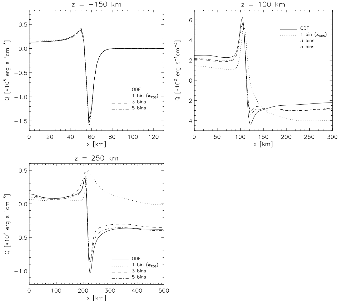
Figure 4.18: Horizontal profiles of Q_{\text{rad}} at three different heights in the 2D atmosphere with an embedded flux sheet. x = 0 corresponds to the symmetry axis of the sheet.
