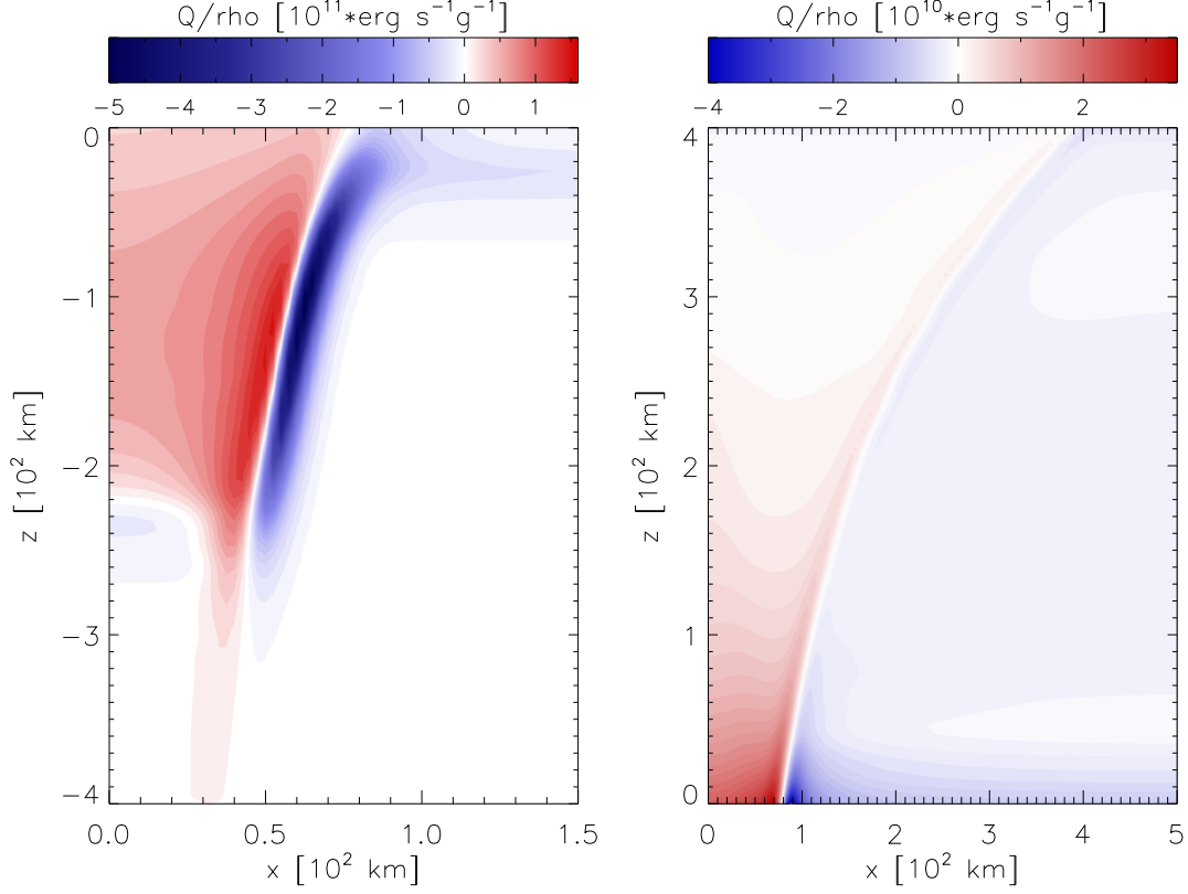
Figure 4.17: Q_{\text{rad}}/\rho for the ODF based reference solution in a magnetic flux sheet model. The left and right panels show the lower part ( z < 0 ) and upper part ( z > 0 ) of the sheet, respectively.
