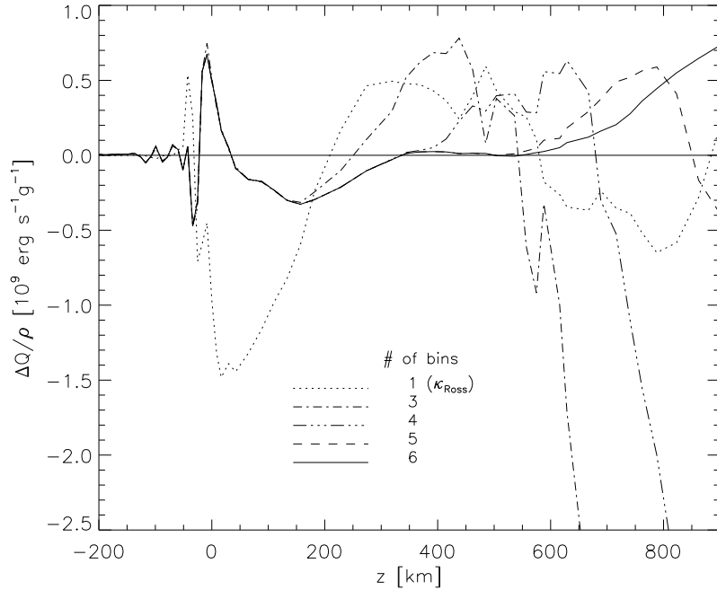
Figure 4.10: (Q - Q_{\text{ODF}})/\rho as a function of height z . The grey solution and four \tau -sorted multi-bin models with 3,4,5, and 6 frequency bins are shown. The spacing between threshold levels separating the bins is \Delta \log \tau_{5000} = 1.5 , and the lowest level is \log \tau_{5000} = 0 for all multi-bin cases.
