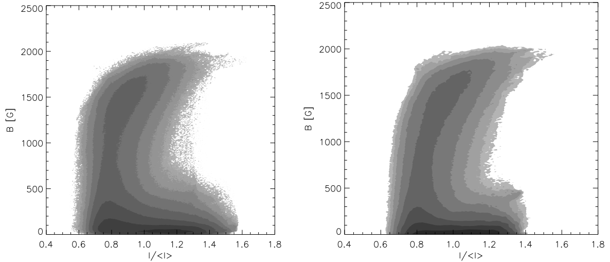
Figure 5.30: Correlation diagrams (joint PDFs) of magnetic field strength at z = 0 versus emergent intensity for the 200-G runs. Left: simulation run with grey radiative transfer. Right: run with four-bin opacity binning. The non-grey radiative transfer reduces the contrast of the nonmagnetic regions, thus enhancing the contrast of magnetic elements relative to the granules.
