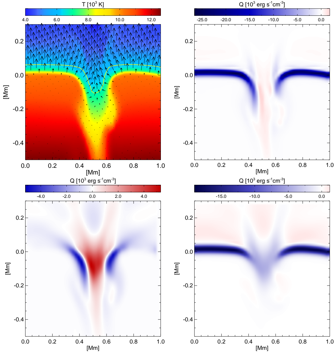
Figure 5.14: Vertical cut through the sheet-like magnetic structure shown in Fig. 5.13. Top left: color-coded temperature and radiative flux vectors; the yellow line indicates the level \tau_{\text{Ross}} = 1 . Top right: radiative heating rate, Q_{\text{rad}} . Bottom left: horizontal radiative energy exchange. Bottom right: vertical radiative energy exchange.
