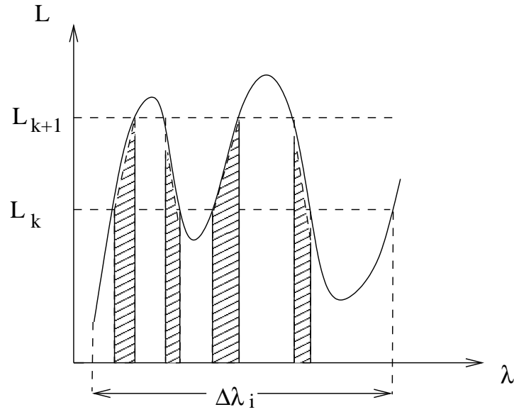
Figure 4.4: Sorting of wavelengths according to a discretization of L . The hatched areas mark those parts of the ODF interval \Delta\lambda_i for which the opacity values lie in the interval [L_k, L_{k+1}[ . They are subsequently reordered to form subinterval \Delta\lambda_{i_j(k)} .
