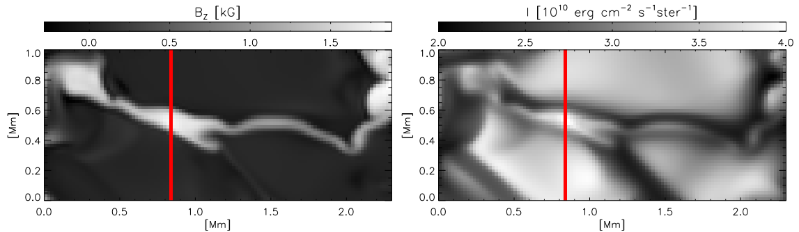
Figure 5.13: Vertical field strength at z = 0 (left) and intensity map (right) for a sheet-like magnetic structure. The red line indicates the position of the cut shown in Fig. 5.14.
