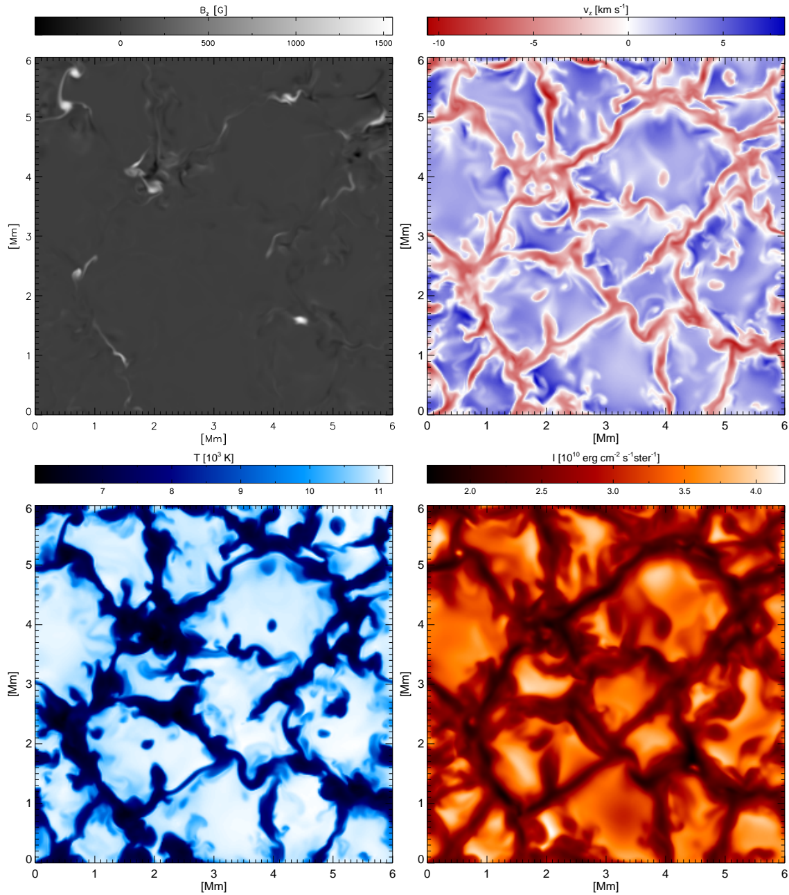
Figure 5.21: Map of frequency-integrated intensity (lower right) and horizontal cuts at the the average geometrical height corresponding to optical depth unity of (clockwise from bottom left) temperature, vertical magnetic field and vertical velocity for the run with an average vertical field strength of 10 G.
