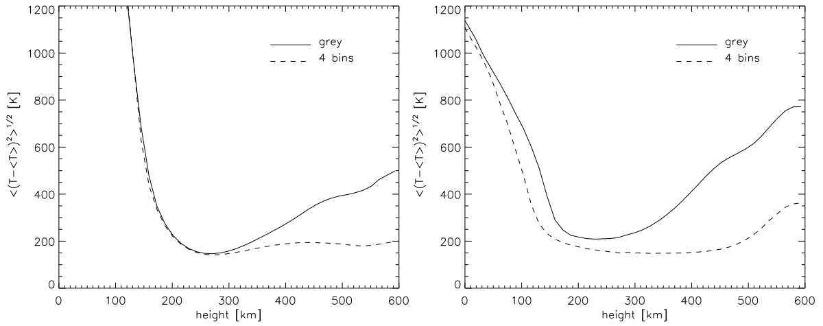
Figure 5.27: Vertical profiles of horizontal temperature fluctuations for the grey and non-grey simulation runs for the height range above z = 0 . Left: fluctuations in weak-field regions with |\mathbf{B}| < 250 G; Right: same in strong-field regions with |\mathbf{B}| > 250 G. The non-grey radiative energy exchange strongly reduces temperature fluctuations in the upper layers of the computational domain, particularly so in regions of strong magnetic field.
