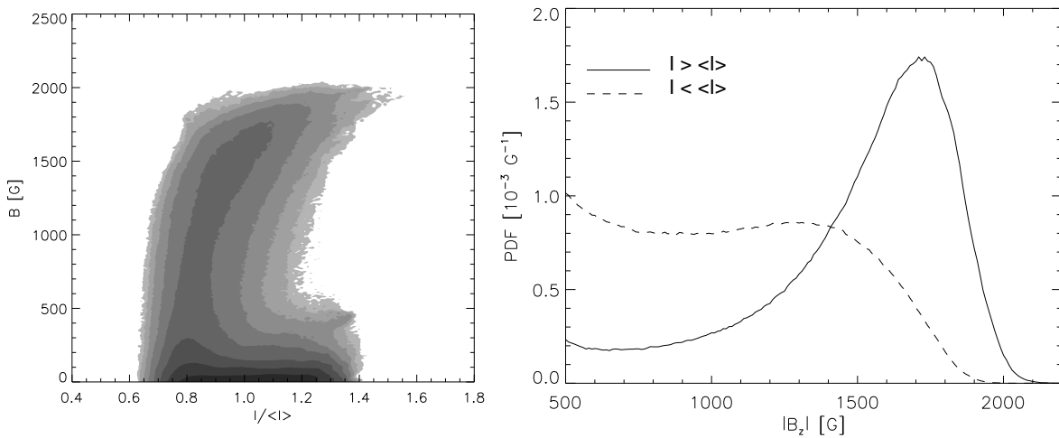
Figure 5.12: Left: Correlation diagram (joint PDF) between magnetic field strength and brightness. The grey-shading indicates the probability density on a logarithmic scale (spaced apart by 0.5 on the \log_{10} -scale). Right: Probability distribution functions of the magnetic field strength inside the magnetic network ( |B_z| > 500 G), for regions brighter and darker than average, respectively.
