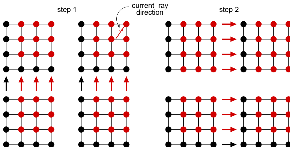
Figure 4.3: A 2D example for the information exchange between four adjacent subdomains, for a ray pointing into the upper right quadrant. After the subdomains have been traversed independently and simultaneously, each process sends the updated intensities to its neighbour in the downwind direction. Black circles represent old values, red circles contain updated information. Likewise, black and red arrows transfer, respectively, old and new data. For each coordinate direction, the communication is performed in a separate step. After the second step the values in the top right subdomain are completely updated.
