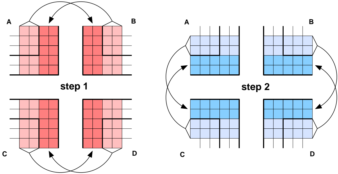
Figure 3.2: Two-step communication between four adjacent processes A to D in two dimensions. Source regions are shaded in light colors, target regions in dark colors.
