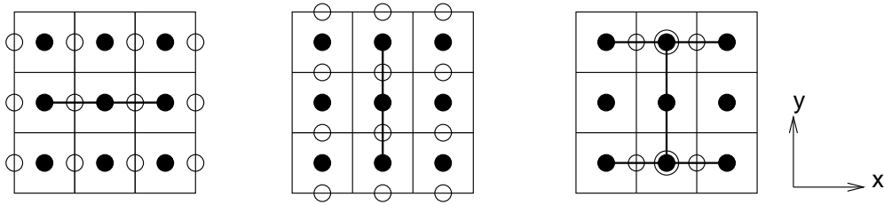
Figure 3.3: The numerical stencil for the artificial diffusivities. Empty circles indicate the staggered grid on which the hyperdiffusive coefficients are defined. Left and middle panel: grid and stencil for the terms \partial_x(\nu\partial_x u) and \partial_y(\nu\partial_y u) , respectively. Right panel: stencil for the term \partial_y(\nu\partial_x u) with mixed derivatives.
