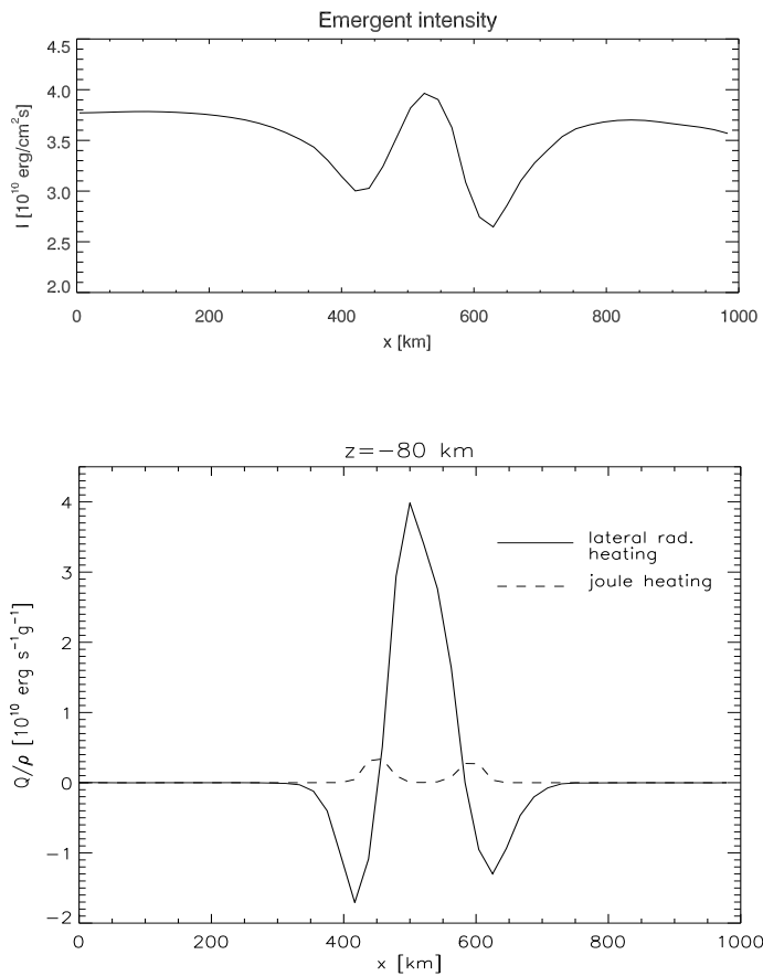
Figure 5.16: Radiative properties of the magnetic sheet shown in Fig. 5.13. Upper panel: Emergent intensity along the cut marked in Fig. 5.13. Lower panel: The solid line shows along the same cut the heating rate due to horizontal influx of radiation energy into the sheet, Q_{\text{hor}} , at a depth of 80 km below z = 0 . The dashed line shows the joule heating occurring at the sheet boundaries at the same depth.
