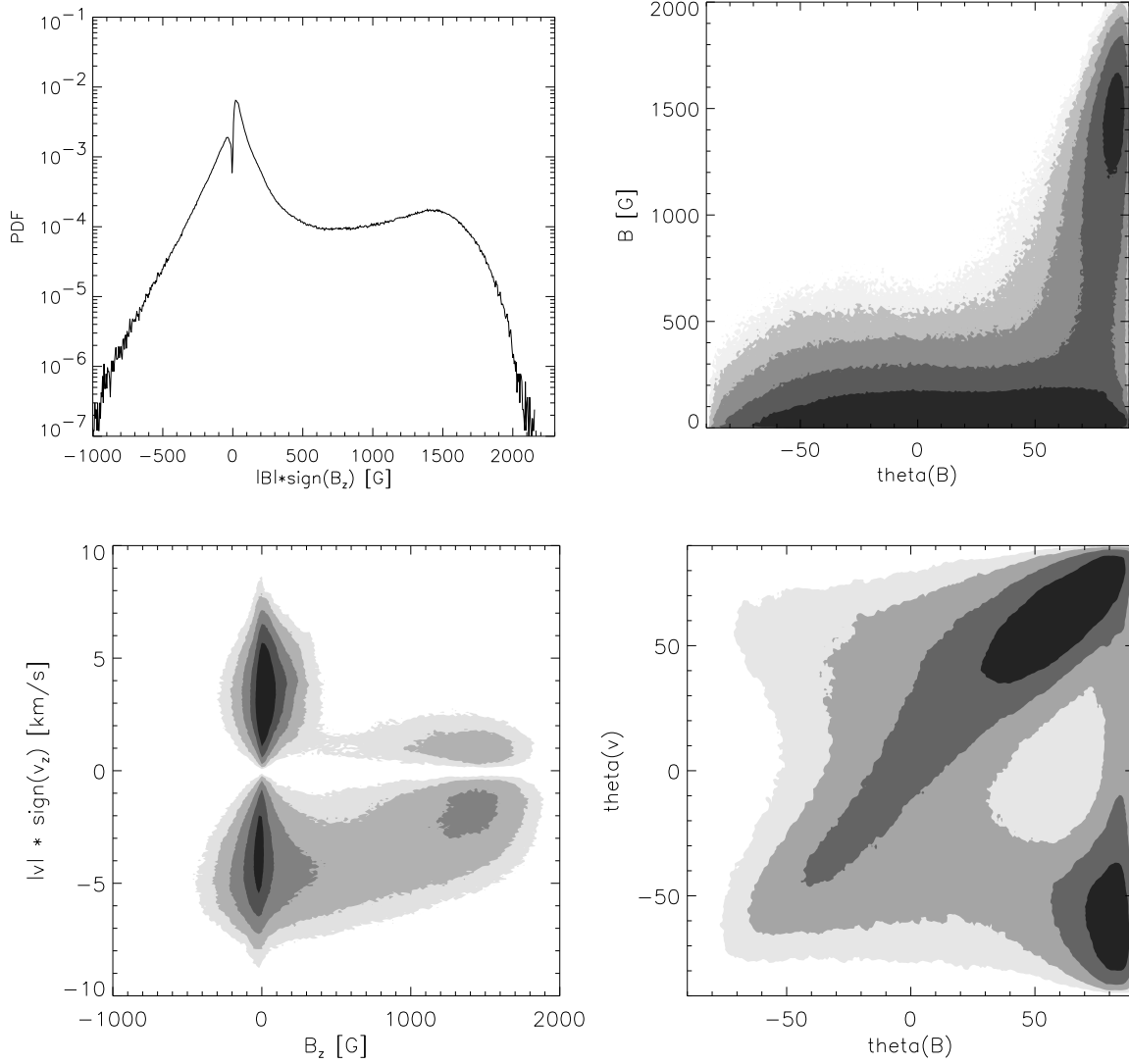
Figure 5.4: Statistical properties of a layer of 112 km thickness around continuum optical depth unity. Upper left: probability distribution (PDF) of the field strength, signed with the vertical orientation of the field vector. Upper right: joint PDF of field strength and the inclination angle of \mathbf{B} with respect to the horizontal, \theta(\mathbf{B}) . Lower left: joint PDF of flow velocity, multiplied with the sign of its vertical component (upflows are positive), and field strength. Lower right: joint PDF of the inclination angles of the flow, \theta(\mathbf{v}) , and of the magnetic field, \theta(\mathbf{B}) . The grey-scaling indicates the probability density on a logarithmic scale.
