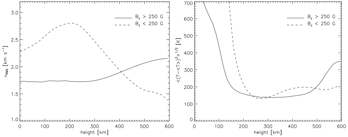
Figure 5.8: Left panel: rms horizontal velocity in regions of strong and weak magnetic field as function of height. A height-independent threshold value of 250 G was chosen. Right panel: rms temperature fluctuations inside and outside strong field regions.
