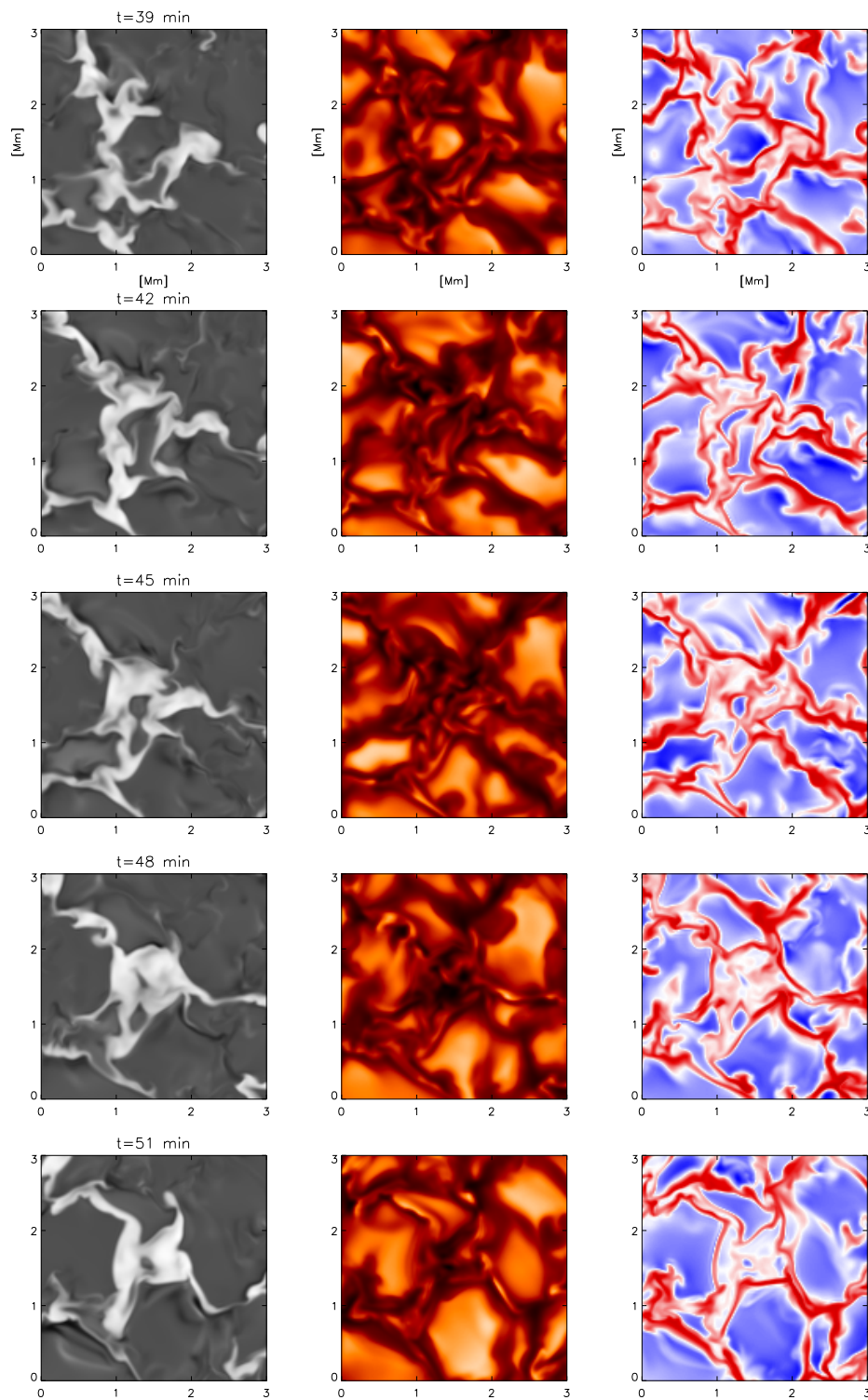
Figure 5.17: Time series of vertical magnetic field (left), intensity (middle), and vertical velocity (right) during the formation of a micropore. An initially bright, small granule is squeezed out of existence by its neighbours. As it shrinks, the magnetic field surrounding it forms a small pore which appears dark in the intensity picture.
