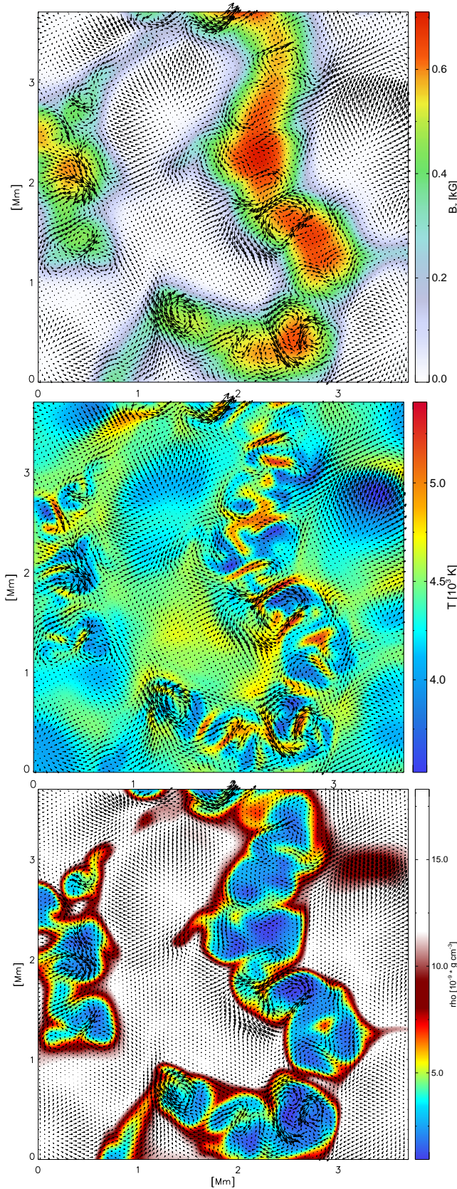
Figure 5.9: Upper panel: vertical magnetic field (color-coded) with superimposed horizontal velocity field for a horizontal slice near the top of the box ( z = 540 km). Only a part of the computational domain is shown. Middle panel: the same region with color-coded temperature. Lower panel: color-coded density. In the upper parts of the simulation box, strong horizontal whirl-flows with maximum amplitudes around 10 \text{ km s}^{-1} occur inside magnetic field structures. They are accompanied by strong temperature fluctuations. These fluctuations are correlated with fluctuations of density, suggesting that they are caused by adiabatic expansion and compression.
