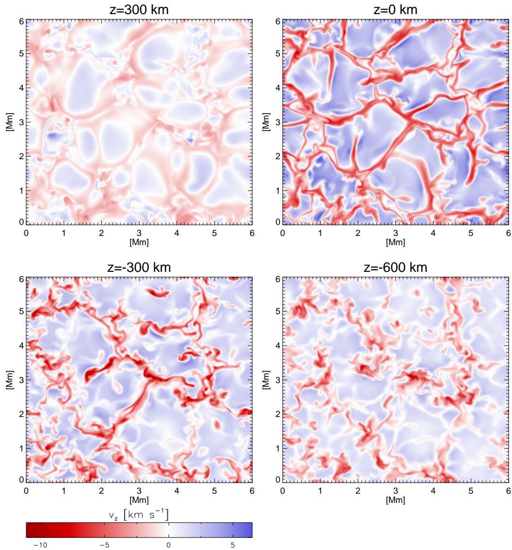
Figure 5.6: Horizontal cuts of vertical velocity at four different height levels. With increasing depth the downflow lanes tend to fragment into more isolated downdrafts. On the whole, however, the meso-scale downflow network can be identified over the complete height range of the computational domain.
