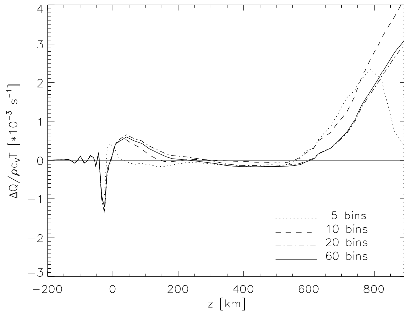
Figure 4.23: Same as Fig. 4.22, for \tau_{\text{ref}} = 0.01
