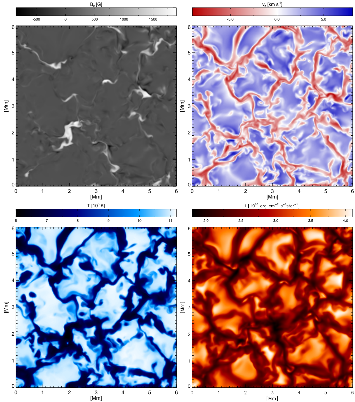
Figure 5.24: Map of frequency-integrated intensity (lower right) and horizontal cuts at the the average geometrical height corresponding to optical depth unity of (clockwise from bottom left) temperature, vertical magnetic field and vertical velocity for the run with an average field strength of 50 G.
