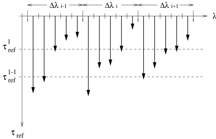
Figure 4.6: Schematic illustration of the \tau -sorting procedure using ODFs. Within each ODF interval \Delta\lambda_i , the ODF steps \Delta\lambda_{ij} are sorted to frequency bins \Omega_l , depending on the height where \tau_{ij} = 1 is reached (indicated by bold arrows).
