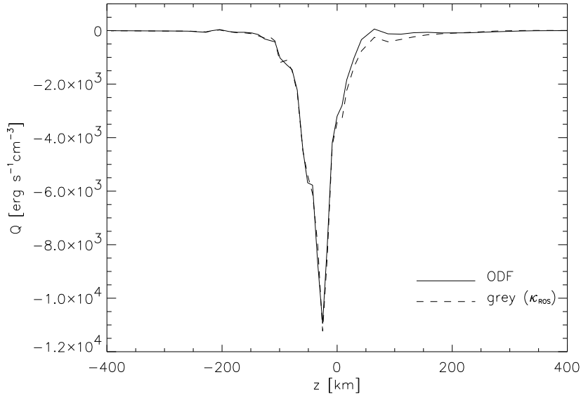
Figure 4.7: The total radiative heating rate as a function of geometrical height for the 1D atmosphere of Maltby et al. (1986). The ODF solution and the grey case with the Rosseland mean opacity are shown. In the height range between z = 0 and z = 200 km, the line opacities lead to a backwarming effect of the ODF case relative to the grey one. z = 0 corresponds to the continuum optical depth \tau_{5000} = 1 .
