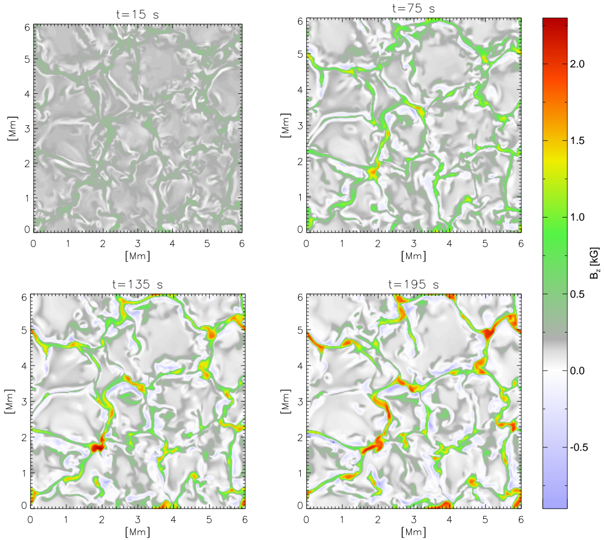
Figure 5.2: Time series of the vertical magnetic field at z = 0 , covering the first three minutes of the magnetic phase. After roughly one turnover time the magnetic flux is swept into the downflow regions and forms a slowly evolving “mesoscale” network of concentrated magnetic structures.
