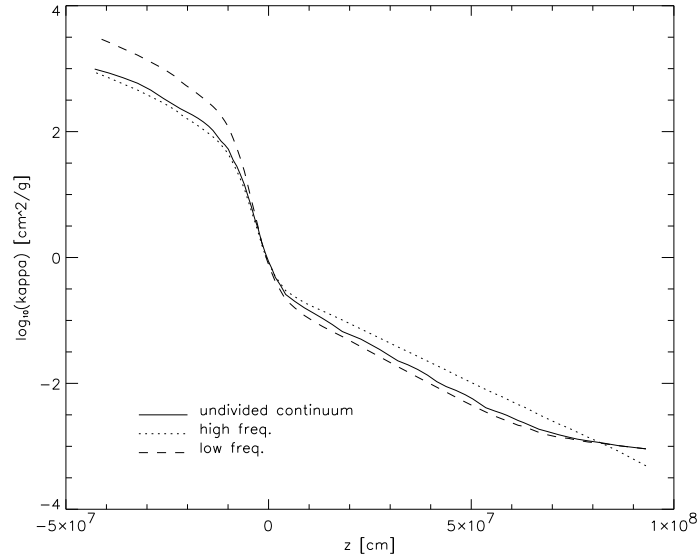
Figure 4.14: The opacity of the unsplit continuum (solid) and the low- and high-frequency sub-bins (dashed and dotted) as a function of height for a 5-bin model without and with frequency-split continuum bin, respectively. The curve for the unsplit bin closely follows the lower of the two sub-bin curves.
