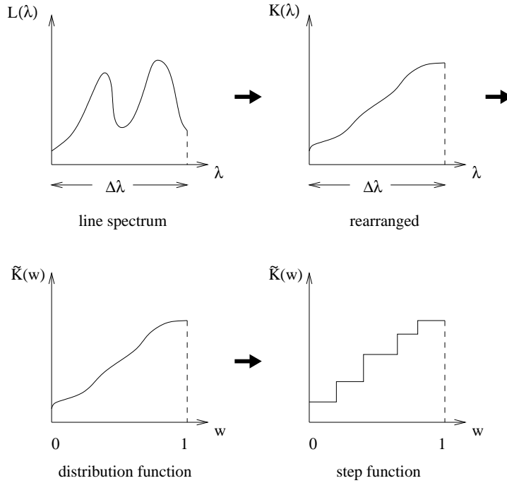
Figure 4.5: From the wavelength-dependent opacity to the tabulated ODF: Within ODF interval \Delta\lambda , the detailed line spectrum is rearranged to form a monotonically increasing function. The corresponding integral probability distribution is then approximated by a step function.
