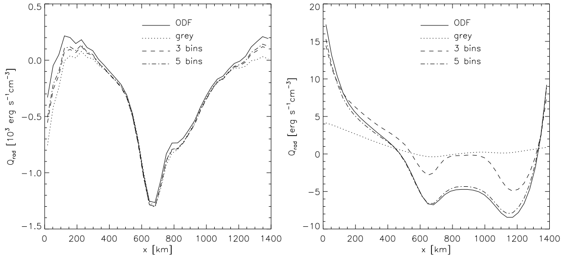
Figure 4.20: Horizontal profiles of Q_{\text{rad}} for a snapshot from a 2D simulation, at heights of 100 km (left) and 500 km (right) above \tau_{5000} = 1 .
