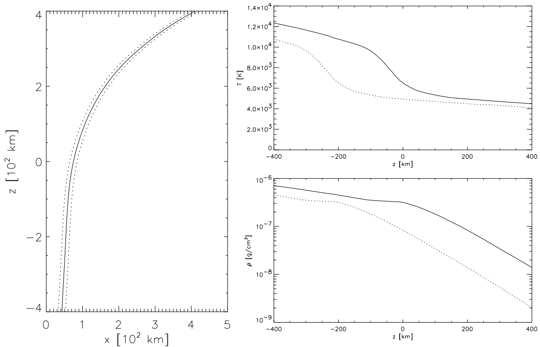
Figure 4.16: Left panel: The solid line marks the boundary between sheet and surrounding atmosphere; only the right half of the sheet is shown. The dotted lines are shifted by 10 km in the horizontal direction. Right panels: Temperature (top) and density (bottom) as function of height z on the symmetry axis ( x = 0 ) of the magnetic sheet (dotted) and in the exterior at x = 500 km (solid).
