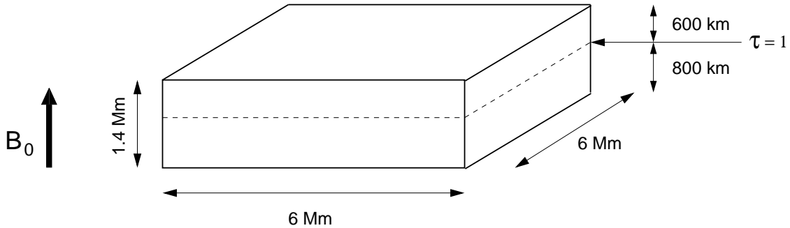
Figure 5.1: Geometrical setup of the simulation runs. The vector \mathbf{B}_0 indicates the vertical homogeneous magnetic field introduced into the hydrodynamic convection at the beginning of the magnetic phase.
