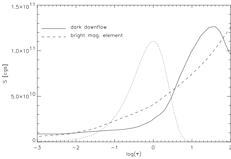
Figure 5.15: Solid line: Vertical profile of the frequency-integrated Planck function (on the \log \tau_{\text{Ross}} scale) for the dark lane ( x = 630 km in Figs. 5.13 - 5.16) next to the magnetic sheet. Dashed line: same for the intensity maximum inside the sheet at x = 520 km. The dotted line shows the contribution function for the vertically emergent intensity in arbitrary units.
