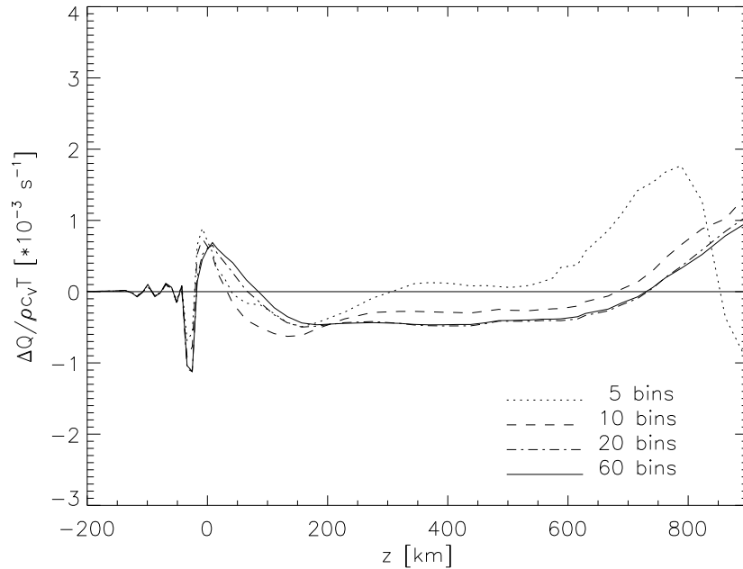
Figure 4.21: Rate of change of the internal energy due deviations of Q from the ODF reference solution as a function of height. Shown are results for \tau -sorted models with different numbers of bins.
