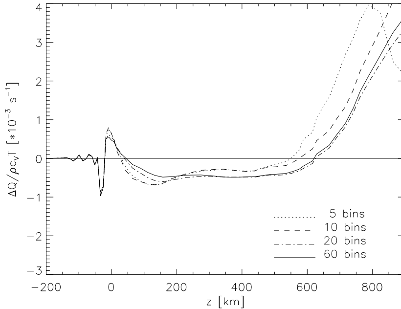
Figure 4.22: Same as Fig. 4.21, but for \kappa -sorting with a sorting parameter of \tau_{\text{ref}} = 0.1 .
