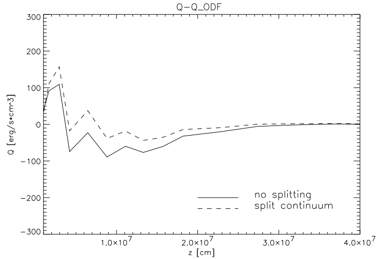
Figure 4.15: Q - Q_{\text{ODF}} for the 5-bin case with and without continuum-splitting. For z > 30 km, the solution with splitting yields the better approximation to the ODF reference solution.
