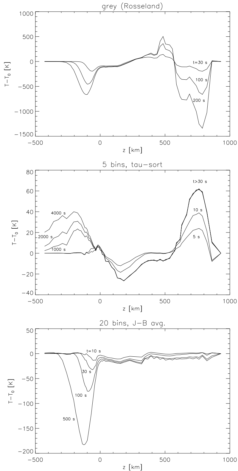
Figure 4.27: Change in temperature for different times after the calculations started. The three panels refer to three different opacity binning models described in the text. Note the different ordinate scales for each panel.
