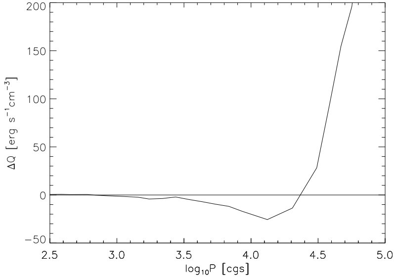
Figure 4.8: The difference Q_{\text{ODF}} - Q_{\text{grey}} plotted against the logarithmic pressure scale; the height in the atmosphere increases towards the left. The transition from backwarming to line-cooling occurs at \log_{10} p \approx 4.35 , which corresponds to z \approx 220 km.
