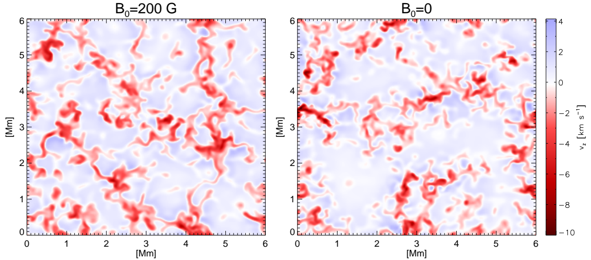
Figure 5.7: Vertical velocity at the bottom of the box ( z = -800 km), for the 200-G run (left panel) and purely hydrodynamic convection without magnetic field (right panel). In the non-magnetic case, downdrafts are stronger and more isolated, and on average the area of connected updrift-regions is larger.
