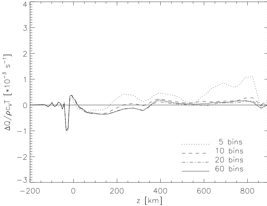
Figure 4.25: Same as Fig.4.21, for a \tau -sorted model where the Planck mean has been replaced in optically thin regions by the J - B mean described in the text.
