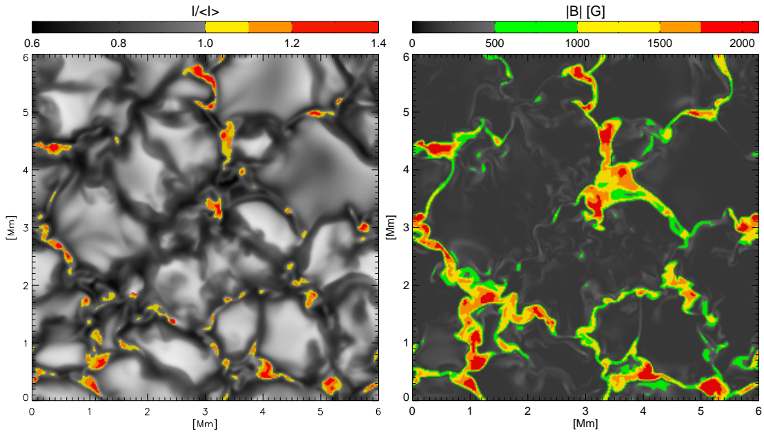
Figure 5.11: Left: Intensity map. Magnetic structures with |\mathbf{B}| > 500 G and above-average intensity are colored. Right: colored map of magnetic field strength at z = 0 . The brightest magnetic structures are preferentially associated with strong fields around 2000 G.
