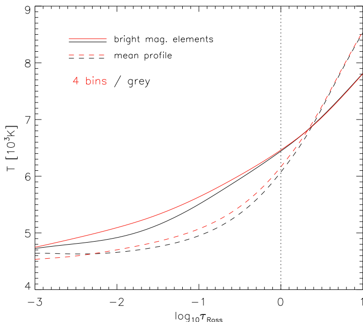
Figure 5.33: Solid lines: vertical temperature profiles inside magnetic structures with above-average brightness. Dashed lines: mean temperature profiles of the whole simulated domain. Red lines correspond to the non-grey simulation run, black ones to the grey run.
