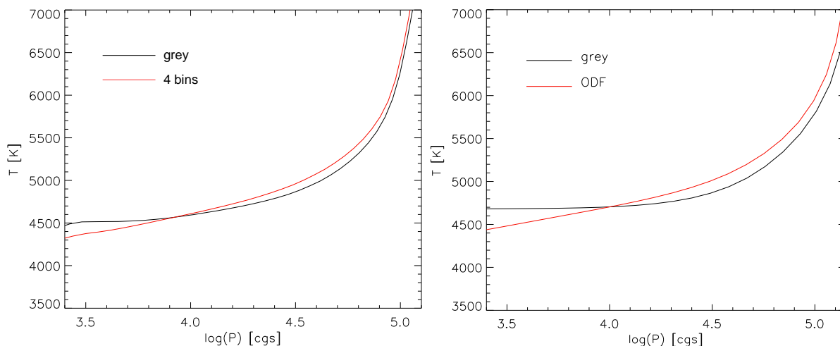
Figure 5.26: Left panel: Average vertical temperature profiles for the 200-G simulation runs with grey and four-bin radiative transfer, respectively. Right panel: temperature profiles of plane-parallel solar model atmospheres obtained from the ATLAS9 code, using Rosseland opacities and Opacity Distribution Functions, respectively.
