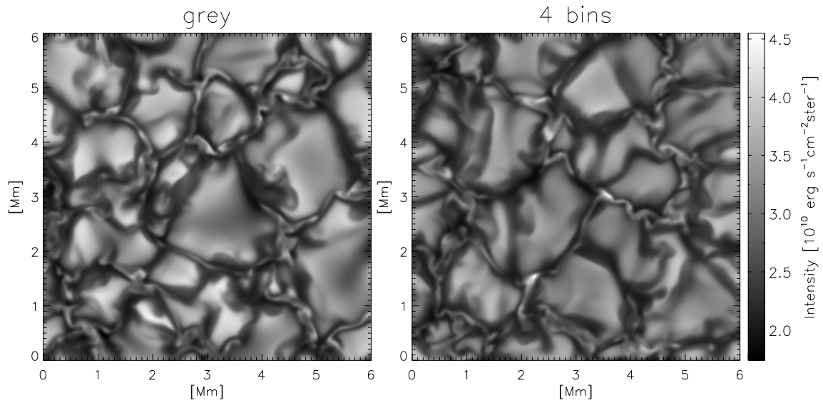
Figure 5.29: Maps of frequency-integrated intensity for the grey (left) and non-grey (right) simulation runs, using the same greyscale table for both pictures. In the non-grey case granules are darker and the overall contrast is reduced. As a result, bright magnetic features stand out more prominently.
