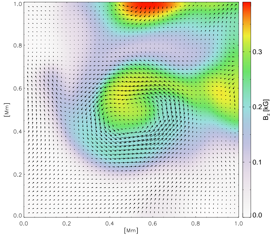
Figure 5.10: Detailed view of the flow and magnetic structure of a flux concentration. Upper panel: velocity field and color-coded vertical magnetic field at z = 540\text{ km} . Lower panel: the same at z = 100\text{ km} .
