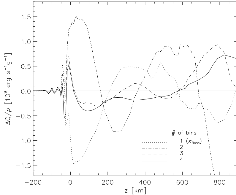
Figure 4.11: (Q - Q_{\text{ODF}})/\rho as a function of height z . The grey solution and \tau -sorted multi-bin models with 2, 3, and 4 frequency bins evenly distributed over the range \log \tau_{5000} < 0 are shown.
