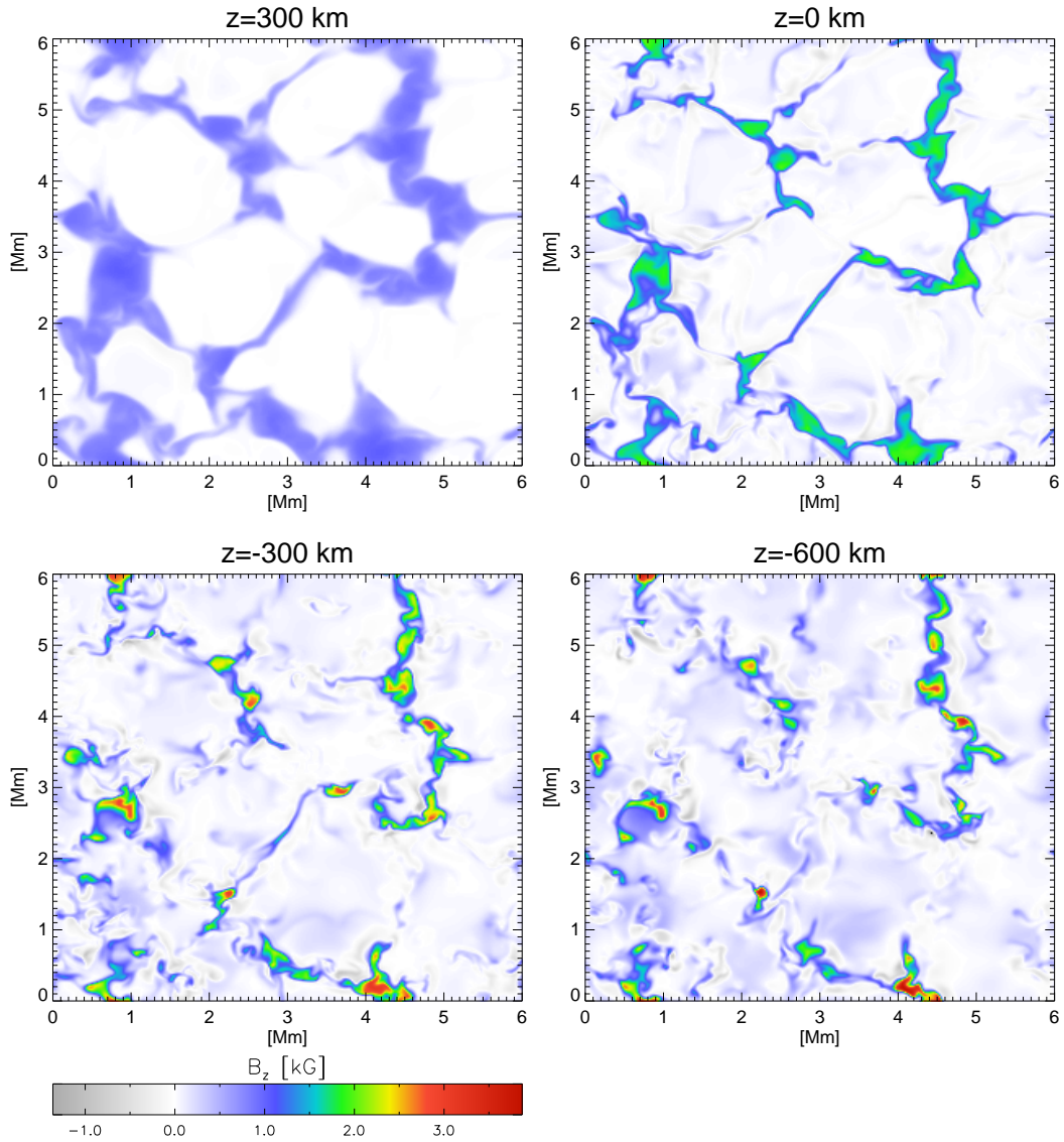
Figure 5.5: Horizontal cuts of vertical magnetic field at four different height levels ( z increases in the upward direction). With increasing depth the magnetic network becomes increasingly fragmented and the flux is concentrated in more isolated structures of high field strength. The mesoscale pattern persists throughout the complete height range.
