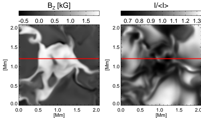
Figure 5.18: Vertical field strength at z = 0 (left) and intensity map (right) of a micropore. The red line indicates the position of the cut shown in Fig. 5.19
