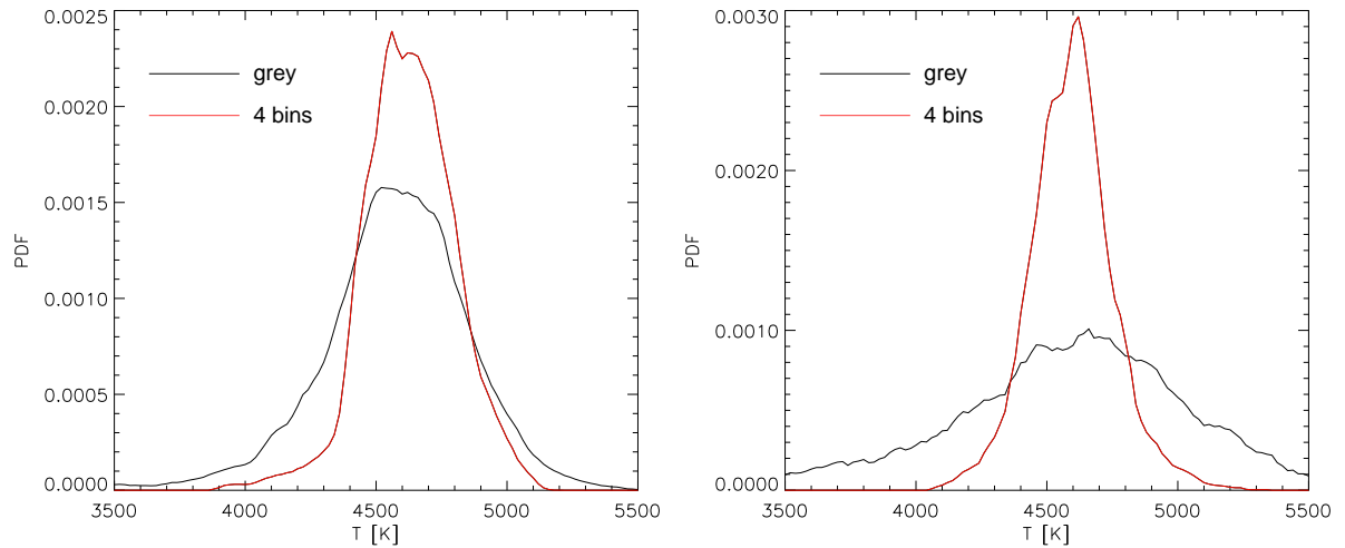
Figure 5.28: Temperature distribution (PDF) at a height of 400 km above z = 0 . Left: distribution in weak-field regions with |\mathbf{B}| < 250 G; Right: same in strong-field regions with |\mathbf{B}| > 250 G.
