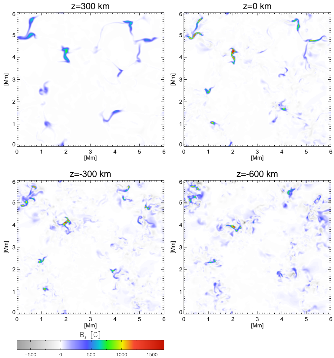
Figure 5.23: Horizontal cuts of vertical magnetic field at four different height levels for the 10-G run. The isolated magnetic field concentrations visible at z = 0 approximately maintain their horizontal positions throughout the whole depth of the computational box.
