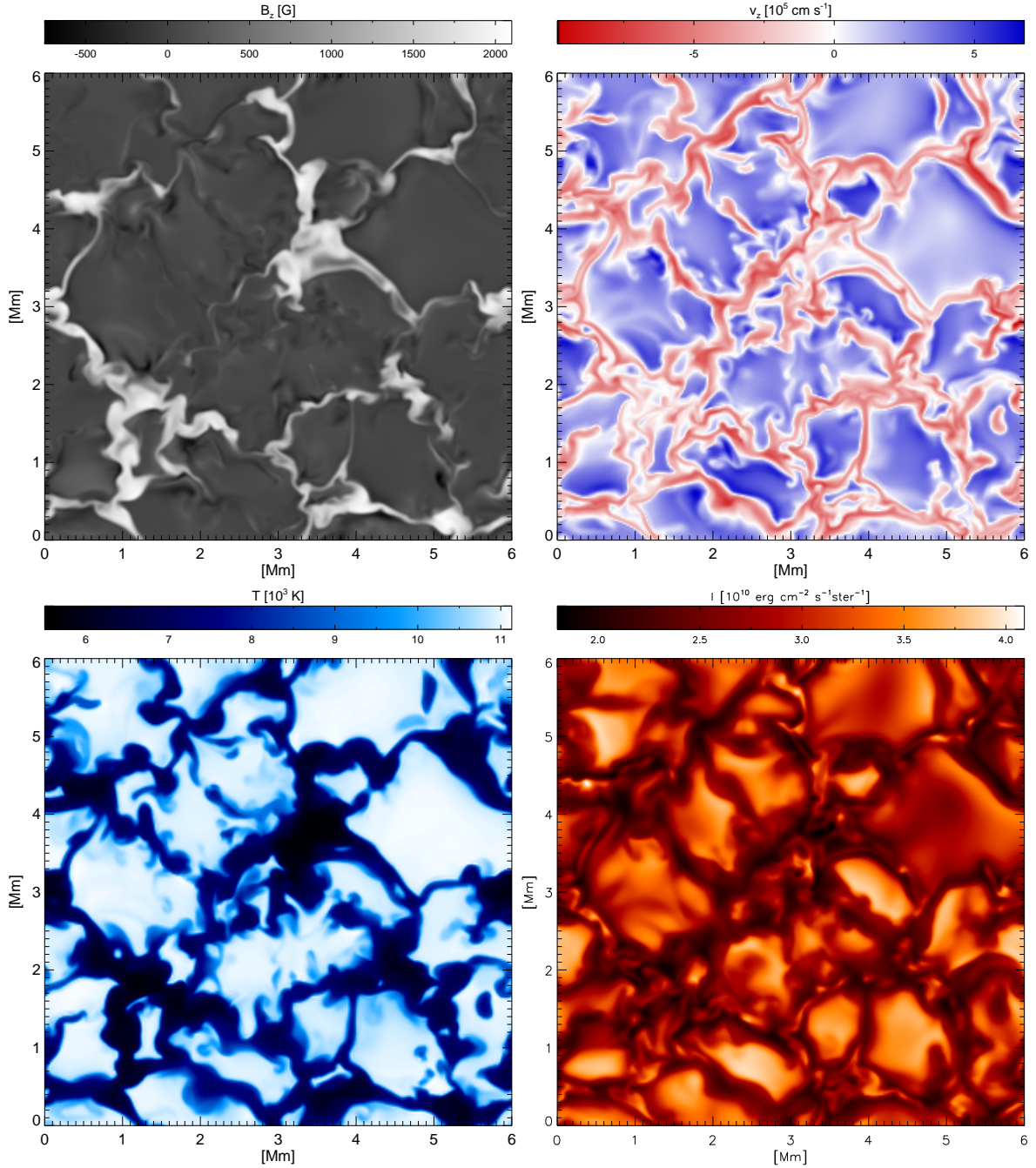
Figure 5.3: Map of frequency-integrated intensity (radiance, lower right) and horizontal cuts at the the average geometrical height corresponding to optical depth unity of (clockwise from bottom left) temperature, vertical magnetic field and vertical velocity. The “mesoscale” network of magnetic field structures is embedded in the network of granular downflows. Larger field concentrations appear dark, while the brightness of small magnetic structures occasionally exceeds the brightness of granules. Most of the domain exhibits “abnormal” granulation with small granules (compared to the “normal” granules in the upper right corner).
