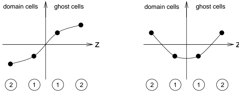
Figure 3.4: Left: A quantity is set to zero on the boundary by filling the ghost cells with values antisymmetric with respect to the neighbouring domain cell values. Right: zero-gradient conditions are realized by filling the ghost cells symmetrically.
